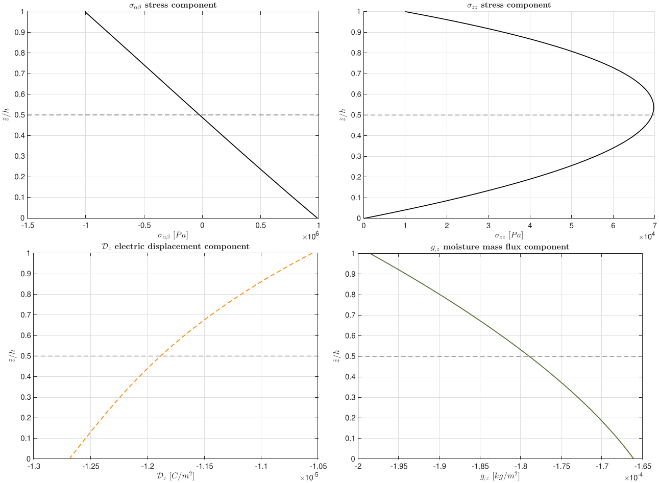
Figure 12 Benchmark B4, 3D- u\text{-}\phi\text{-}\mathcal{M} graphical trends along the thickness direction for the simply-supported multilayered spherical shell in sensor closed circuit configuration ( \bar{P}_{z_t} = 10000 \text{ Pa} , \bar{P}_{z_b} = 0 \text{ Pa} , \bar{\Phi}_t = 0 \text{ A} , \bar{\Phi}_b = 0 \text{ A} , \bar{\mathcal{M}}_t = 1.5 \text{ kg/m}^3 , \bar{\mathcal{M}}_b = 0.5 \text{ kg/m}^3 ) for R_\alpha/h = 10 .
