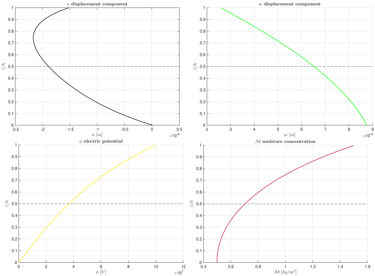
Figure 2 Benchmark B1, 3D- u - \phi - \mathcal{M} graphical trends along the thickness direction for the simply-supported multilayered plate in actuator configuration ( \bar{P}_{zt} = 0 \text{ Pa} , \bar{P}_{zb} = 0 \text{ Pa} , \bar{\Phi}_t = 1 \cdot 10^8 \text{ A} , \bar{\Phi}_b = 0 \text{ A} , \bar{\mathcal{M}}_t = 1.5 \text{ kg/m}^3 , \bar{\mathcal{M}}_b = 0.5 \text{ kg/m}^3 ) for a/h = 4 .
