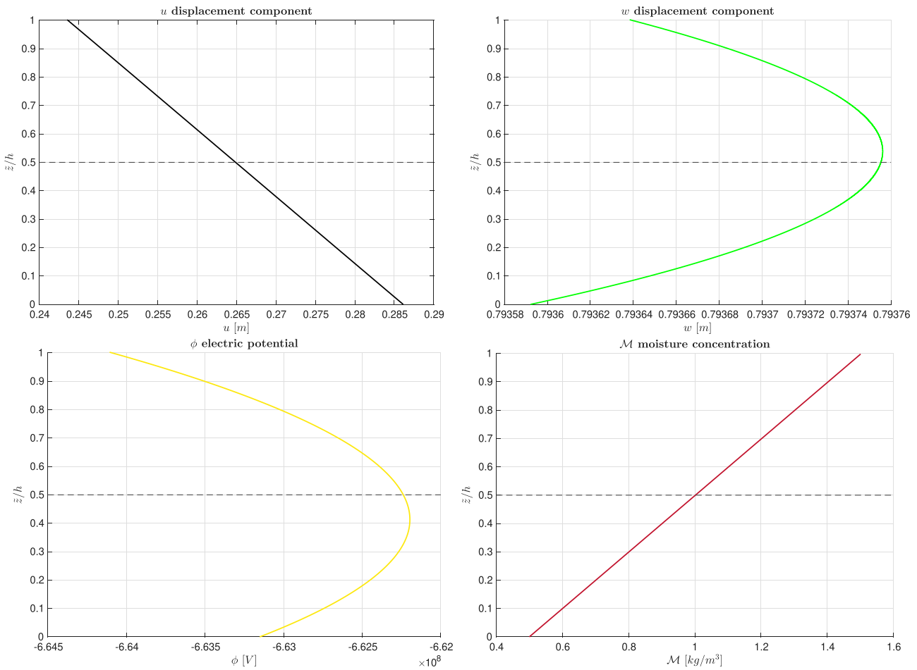
Figure 10 Benchmark B3, 3D- u - \phi - \mathcal{M} graphical trends along the thickness direction for the simply-supported multilayered cylindrical panel in sensor open circuit configuration ( \bar{P}_{zt} = 10000 \text{ Pa} , \bar{P}_{zb} = 0 \text{ Pa} , \bar{D}_{zt} = 0.001 \text{ C/m}^2 , \bar{D}_{zb} = 0 \text{ C/m}^2 , \bar{\mathcal{M}}_t = 1.5 \text{ kg/m}^3 , \bar{\mathcal{M}}_b = 0.5 \text{ kg/m}^3 ) for R_\alpha/h = 50 .
