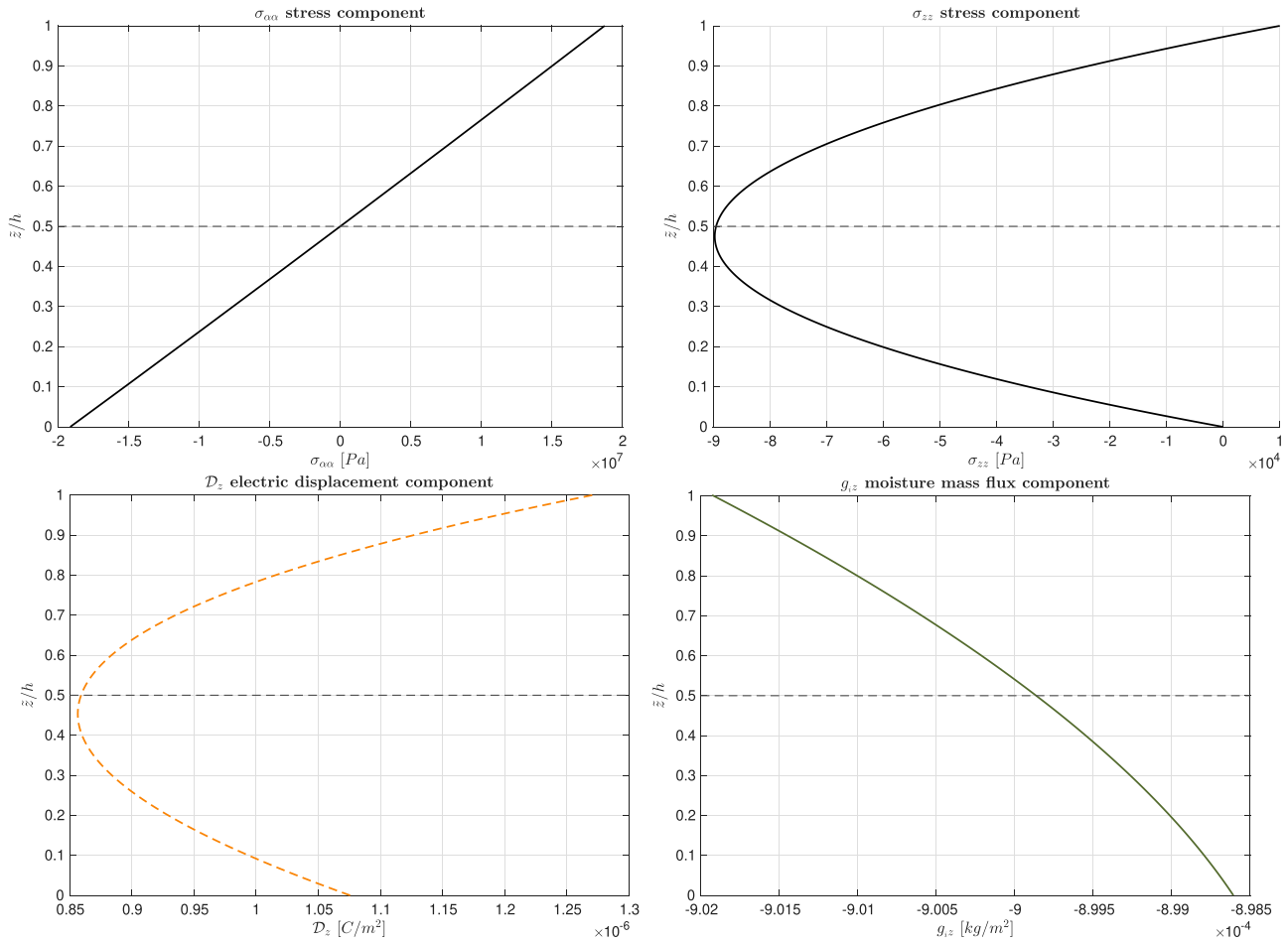
Figure 9 Benchmark B3, 3D- u - \phi - \mathcal{M} graphical trends along the thickness direction for the simply-supported multilayered cylindrical panel in sensor closed circuit configuration ( \bar{P}_{zt} = 10000 \text{ Pa} , \bar{P}_{zb} = 0 \text{ Pa} , \bar{\Phi}_t = 0 \text{ A} , \bar{\Phi}_b = 0 \text{ A} , \bar{\mathcal{M}}_t = 1.5 \text{ kg/m}^3 , \bar{\mathcal{M}}_b = 0.5 \text{ kg/m}^3 ) for R_\alpha/h = 50 .
