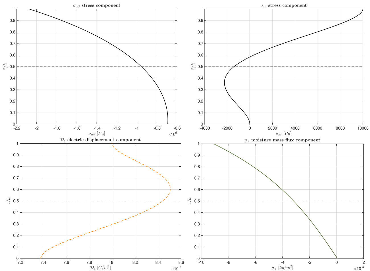
Figure 3 Benchmark B1, 3D- u-\phi-\mathcal{M} graphical trends along the thickness direction for the simply-supported multilayered plate in sensor closed circuit configuration ( \bar{P}_{zt} = 10000 \text{ Pa} , \bar{P}_{zb} = 0 \text{ Pa} , \bar{\Phi}_t = 0 \text{ A} , \bar{\Phi}_b = 0 \text{ A} , \bar{\mathcal{M}}_t = 1.5 \text{ kg/m}^3 , \bar{\mathcal{M}}_b = 0.5 \text{ kg/m}^3 ) for a/h = 4 .
