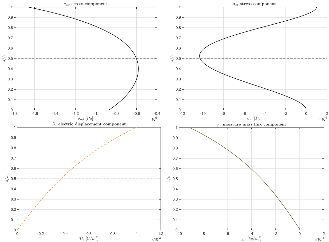
Figure 4 Benchmark B1, 3D- u-\phi-\mathcal{M} graphical trends along the thickness direction for the simply-supported multilayered plate in sensor open circuit configuration ( \bar{P}_{zt} = 10000 \text{ Pa} , \bar{P}_{zb} = 0 \text{ Pa} , \bar{D}_{zt} = 0.001 \text{ C/m}^2 , \bar{D}_{zb} = 0 \text{ C/m}^2 , \bar{\mathcal{M}}_t = 1.5 \text{ kg/m}^3 , \bar{\mathcal{M}}_b = 0.5 \text{ kg/m}^3 ) for a/h = 4 .
