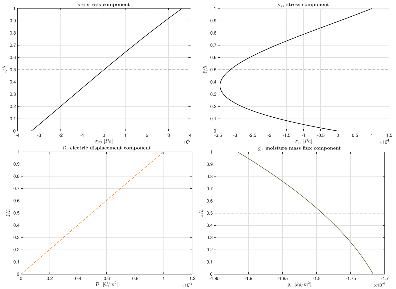
Figure 7 Benchmark B2, 3D- u - \phi - \mathcal{M} graphical trends along the thickness direction for the simply-supported multilayered cylinder in sensor open circuit configuration ( \bar{P}_{zt} = 10000 \text{ Pa} , \bar{P}_{zb} = 0 \text{ Pa} , \bar{D}_{zt} = 0.001 \text{ C/m}^2 , \bar{D}_{zb} = 0 \text{ C/m}^2 , \bar{\mathcal{M}}_t = 1.5 \text{ kg/m}^3 , \bar{\mathcal{M}}_b = 0.5 \text{ kg/m}^3 ) for R_\alpha/h = 10 .
