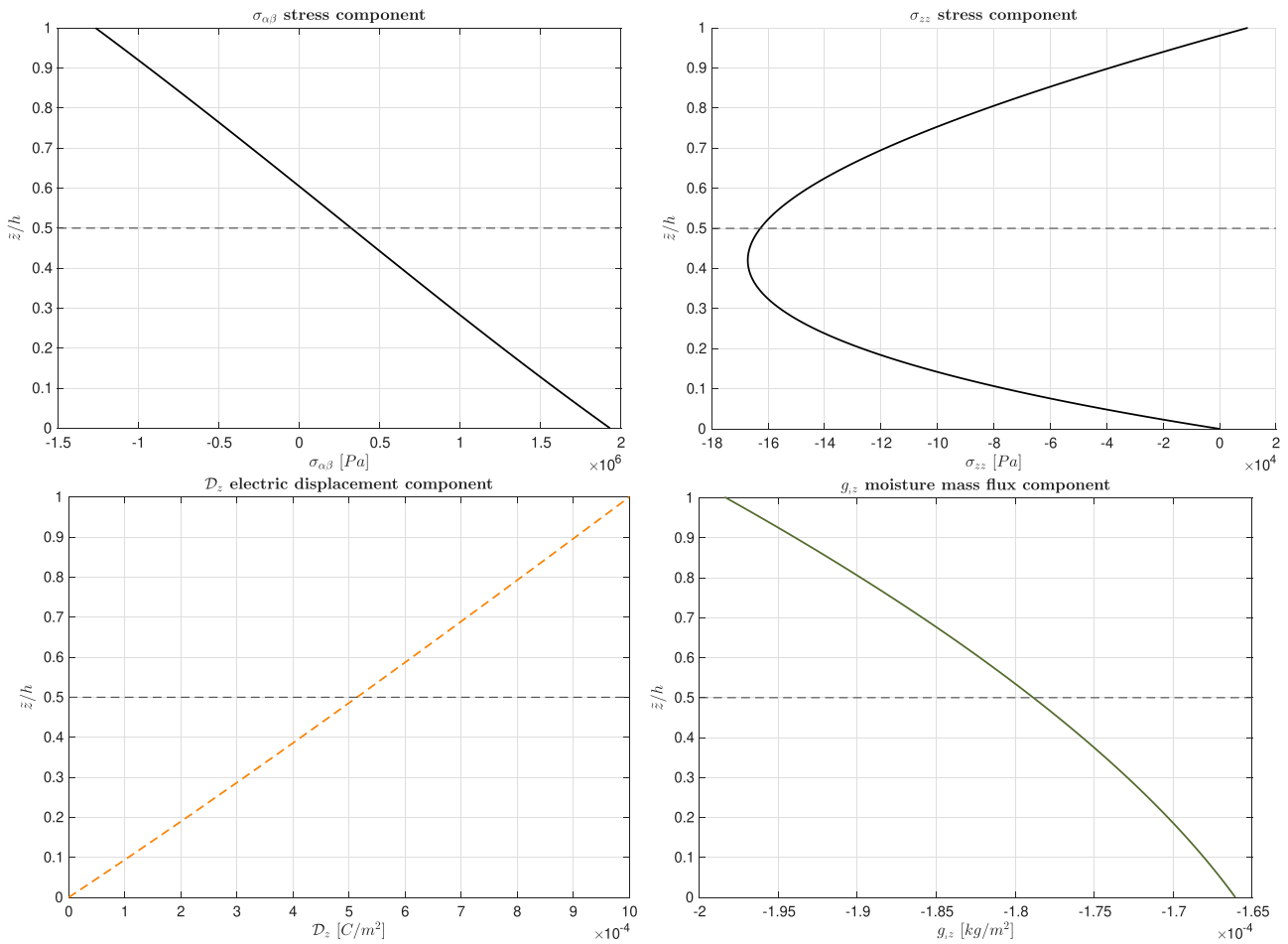
Figure 13 Benchmark B4, 3D- u - \phi - \mathcal{M} graphical trends along the thickness direction for the simply-supported multilayered spherical shell in sensor open circuit configuration ( \bar{P}_{z_t} = 10000 \text{ Pa} , \bar{P}_{z_b} = 0 \text{ Pa} , \bar{D}_{z_t} = 0.001 \text{ C/m}^2 , \bar{D}_{z_b} = 0 \text{ C/m}^2 , \bar{\mathcal{N}}_t = 1.5 \text{ kg/m}^3 , \bar{\mathcal{N}}_b = 0.5 \text{ kg/m}^3 ) for R_\alpha/h = 10 .
