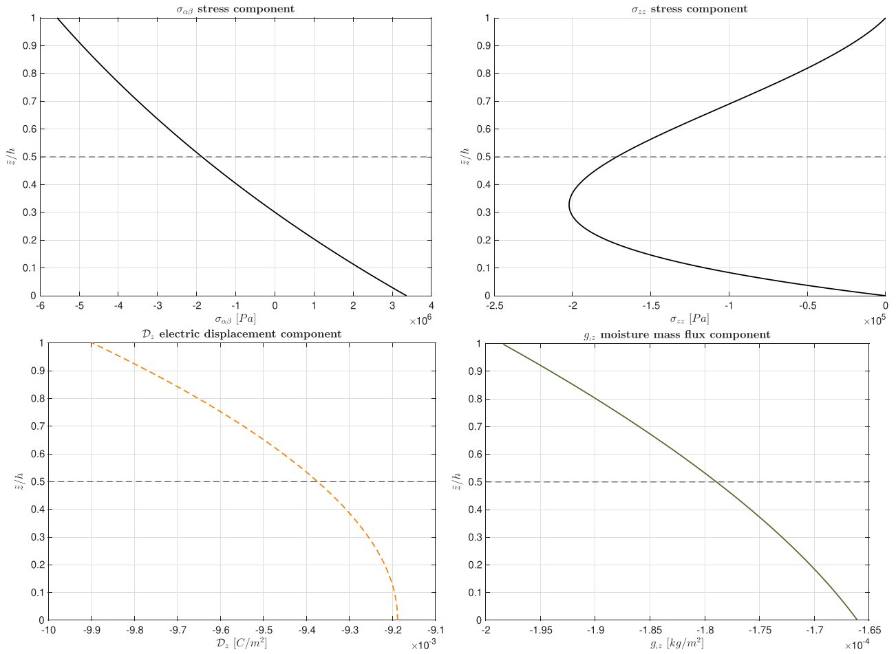
Figure 11 Benchmark B4, 3D- u\text{-}\phi\text{-}\mathcal{M} graphical trends along the thickness direction for the simply-supported multilayered spherical shell in actuator configuration ( \bar{P}_{zt} = 0 \text{ Pa} , \bar{P}_{zb} = 0 \text{ Pa} , \bar{\Phi}_t = 1 \cdot 10^8 \text{ A} , \bar{\Phi}_b = 0 \text{ A} , \bar{\mathcal{N}}_t = 1.5 \text{ kg/m}^3 , \bar{\mathcal{N}}_b = 0.5 \text{ kg/m}^3 ) for R_\alpha/h = 10 .
