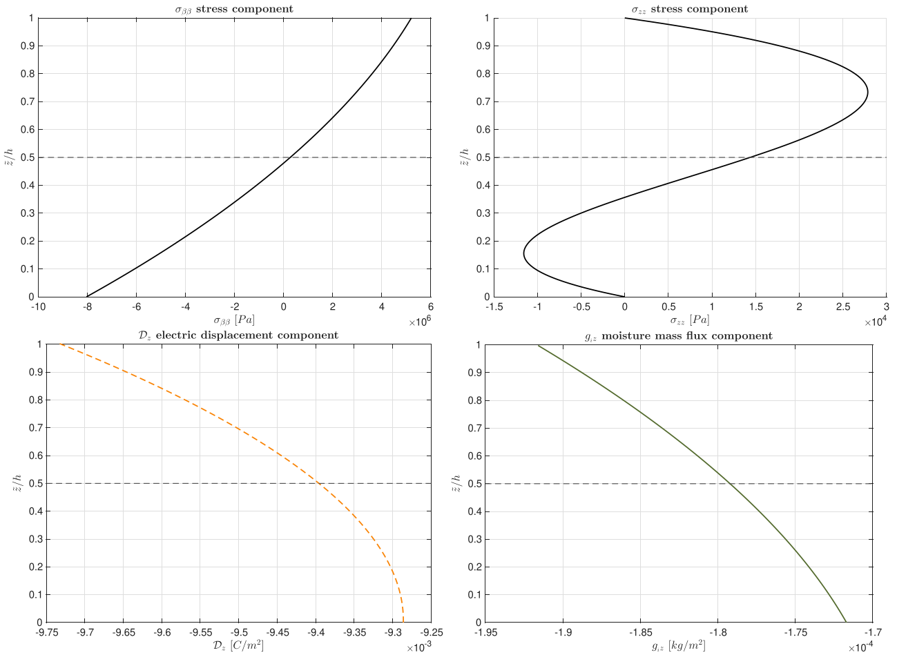
Figure 5 Benchmark B2, 3D- u - \phi - \mathcal{M} graphical trends along the thickness direction for the simply-supported multilayered cylinder in actuator configuration ( \bar{P}_{z_t} = 0 \text{ Pa} , \bar{P}_{z_b} = 0 \text{ Pa} , \bar{\Phi}_t = 1 \cdot 10^8 \text{ A} , \bar{\Phi}_b = 0 \text{ A} , \bar{\mathcal{M}}_t = 1.5 \text{ kg/m}^3 , \bar{\mathcal{M}}_b = 0.5 \text{ kg/m}^3 ) for R_\alpha/h = 10 .
