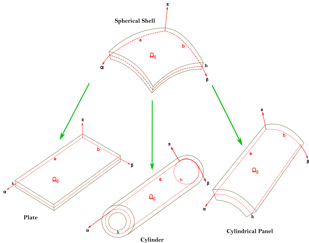
Figure 1 Geometries, mixed curvilinear orthogonal reference system and middle reference surfaces \Omega_0 for assessments and benchmarks. Dotted lines indicate the middle reference surface \Omega_0 . The origin of the mixed curvilinear orthogonal reference system is indicated at the top left corner of each geometry. Spherical shell degenerates in simpler geometries.
