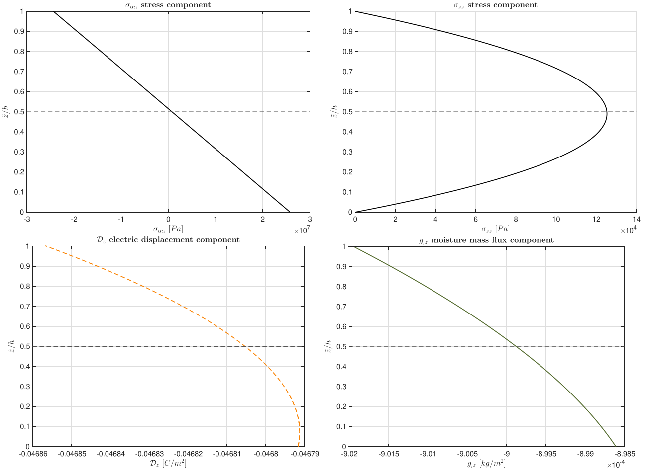
Figure 8 Benchmark B3, 3D- u - \phi - \mathcal{M} graphical trends along the thickness direction for the simply-supported multilayered cylindrical panel in actuator configuration ( \bar{P}_{z_t} = 0 \text{ Pa} , \bar{P}_{z_b} = 0 \text{ Pa} , \bar{\Phi}_t = 1 \cdot 10^8 \text{ A} , \bar{\Phi}_b = 0 \text{ A} , \bar{\mathcal{M}}_t = 1.5 \text{ kg/m}^3 , \bar{\mathcal{M}}_b = 0.5 \text{ kg/m}^3 ) for R_\alpha/h = 50 .
