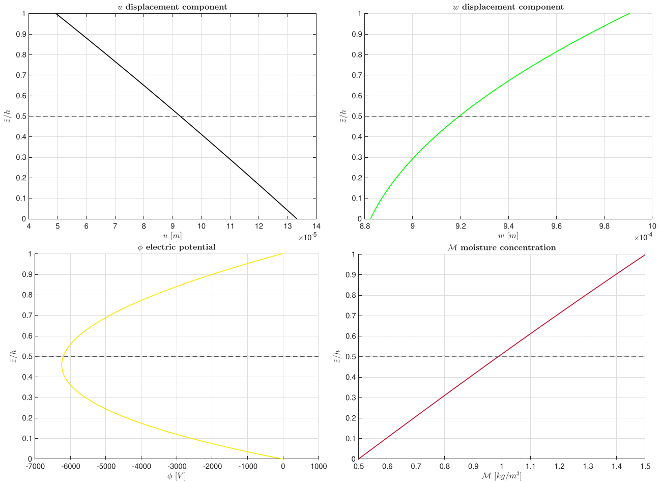
Figure 6 Benchmark B2, 3D- u - \phi - \mathcal{M} graphical trends along the thickness direction for the simply-supported multilayered cylinder in sensor closed circuit configuration ( \bar{P}_{zt} = 10000 \text{ Pa} , \bar{P}_{zb} = 0 \text{ Pa} , \bar{\Phi}_t = 0 \text{ A} , \bar{\Phi}_b = 0 \text{ A} , \bar{\mathcal{M}}_t = 1.5 \text{ kg/m}^3 , \bar{\mathcal{M}}_b = 0.5 \text{ kg/m}^3 ) for R_\alpha/h = 10 .
