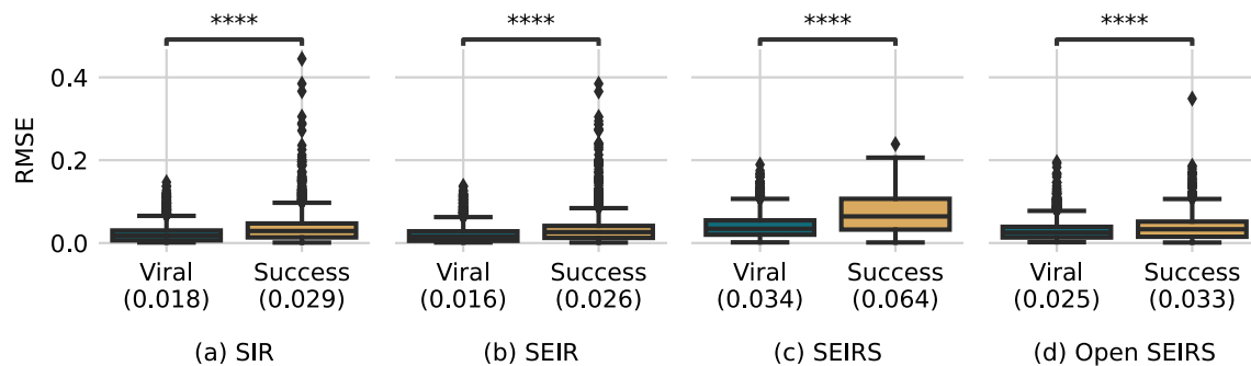
Fig. 2 RMSE for virality and success curves using single epidemic models. Values in parentheses are the median values. Significance is calculated using the Mann–Whitney U test: **** indicates p \leq 0.0001
