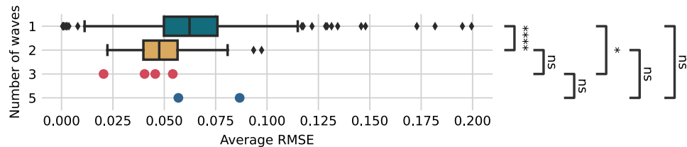
Fig. 5 Average RMSE distribution grouped by the number of identified waves. Significance is calculated using the Mann–Whitney U test: * for 0.01 < p \leq 0.05 ; **** for p \leq 0.0001 ; and ‘ns’ for p > 0.05
