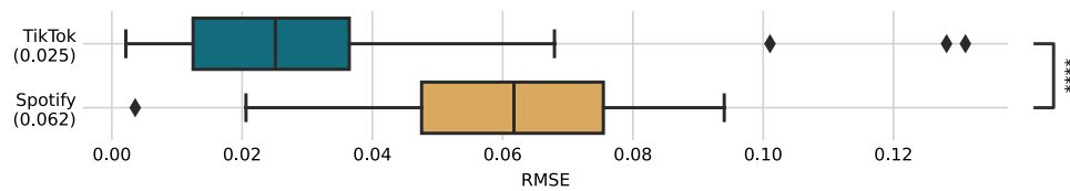
Fig. 13 RMSE for TikTok and Spotify virality curves using the wave-based approach. Values in parentheses are the median values. Significance is calculated using the Mann–Whitney U test: **** for p \leq 0.0001
