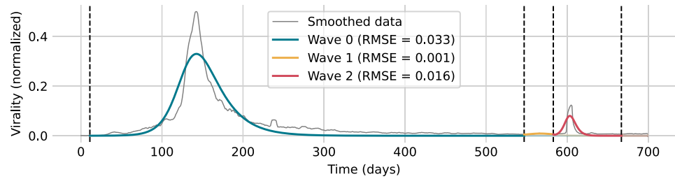
Fig. 11 TikTok virality time series with the wave-based SEIR fit for the song “Heather” by Conan Gray. The vertical dashed lines delimit the waves
