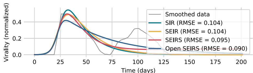
Fig. 3 Model fits for the virality of “Mon Amour - Remix” by Zzoilo and Aitana
