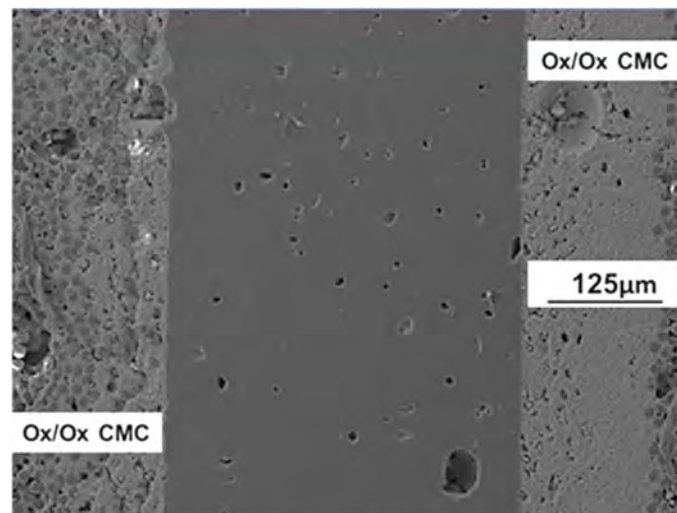
Fig. 6. Cross-section of SACM glass-ceramic joined Ox-Ox CMC after 50 h of thermal ageing at 930 °C in air (from [69]).
