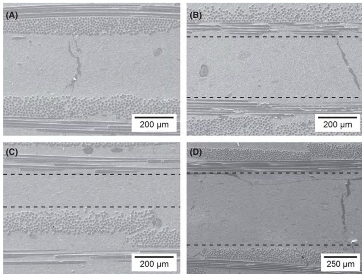
Fig. 12. Cross-sections of N610/AZ composites produced (A) and joining area of gel joint (B), green joint (C), and sintering joint (D). Dashed lines demarcate the joining region (from [75]).
