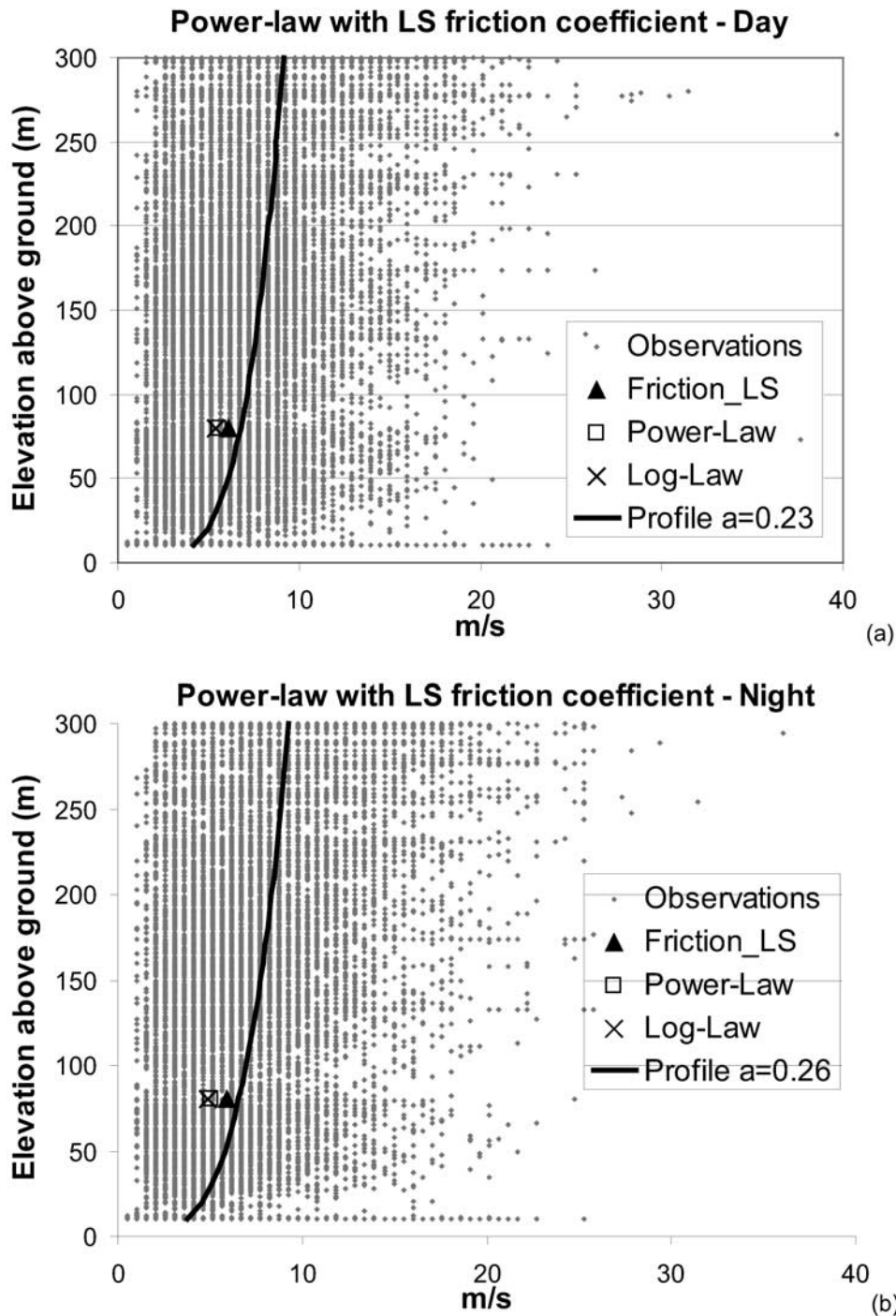
Figure 11. Wind speed observed worldwide in the lowest 300 m, calculated V80 obtained with: \alpha^{LS} (triangle), z_0 = 0.01 (cross), \alpha = 1/7 (square), and profile obtained (a) with the world average \alpha^{LS} = 0.23 (solid line) during the day and (b) with \alpha^{LS} = 0.26 at night.
