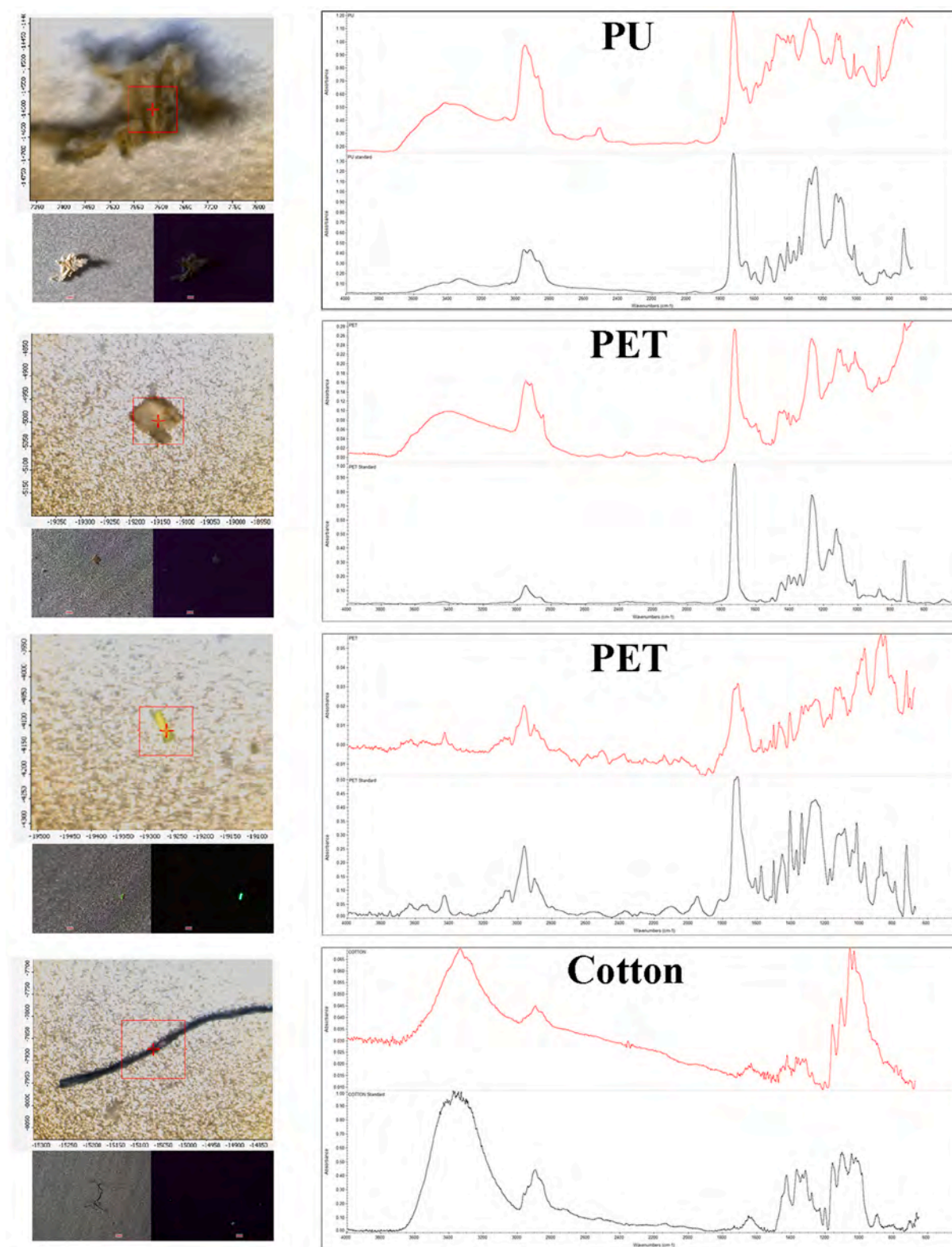
Fig. 4. \mu FTIR spectra of selected microparticles of anthropogenic origin found in the dripping water of the Torri di Slivia cave, Italy., together with their corresponding optical microscope images acquired under both visible and UV light. Images: \mu FTIR particle visualization at the top, optical microscope images at the bottom left, and optical microscope images under UV light at the bottom right.
