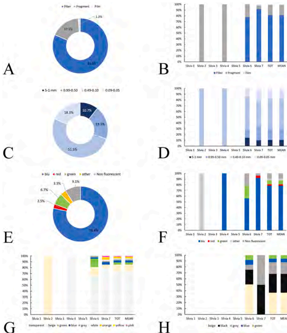
Fig. 5. AMP characteristics in the dripping water of Torri di Silvia cave. A: shape, total; B: shape for each sampling point; C: size, total; D: size for each sampling point; E, fluorescence, total; F: fluorescence for each sampling point; G: colour of fluorescent particles; H: colour of not fluorescent particles.
