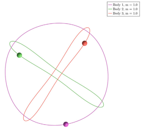
Fig. 4. Solution of the 3-body problem, typically known as Ducati and first discovered in Moore (1993). Its Floquet multipliers show that the orbit is linearly stable.
