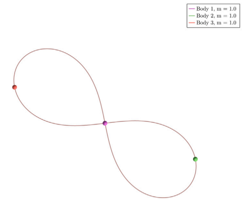
Fig. 3. Figure-eight choreography. The orbit is not a minimiser of the action and has positive Morse index, but its Floquet multipliers lie close to the unit circle, indicating near-linear stability.
