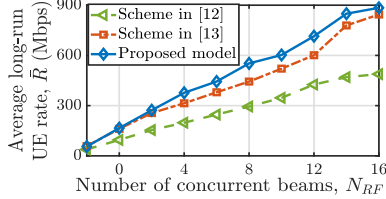
Fig. 6. Comparison of achievable \bar{R} with different schemes.
