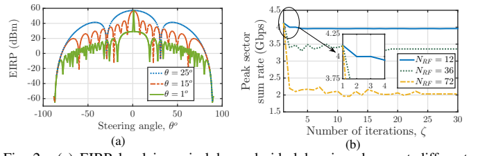
Fig. 2. (a) EIRP level in main-lobe and side-lobes in a beam at different beamwidth. (b) Convergence of peak sector sum rate in an epoch for U = 400 and S = 72 .
