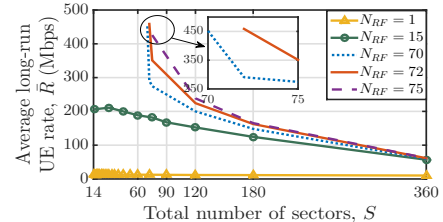
Fig. 4. Illustration of \bar{R} as a function of S for different N_{RF} and U = 400 .
