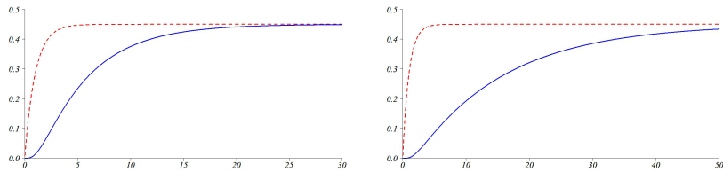
FIGURE 4. Plots of the m_{V_1}(t|v_0, t_0) (red dashed) and m_{V_2}(t|v_0, t_0) (blue solid) for S = 1.5 (on the left) and S = 2 (on the right). The other parameters are as in Fig. 3.
