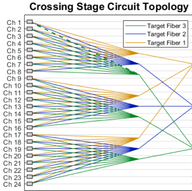
Fig. 6. Interconnect stage topology for a 24 channels device with 3 target output ports.
