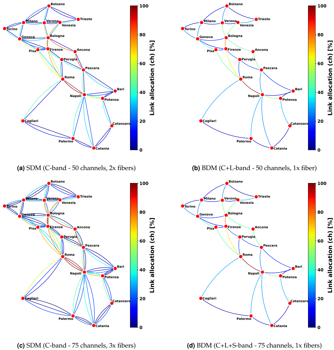
Fig. 18. Italian topology channel allocation comparison - 800G transceiver.
