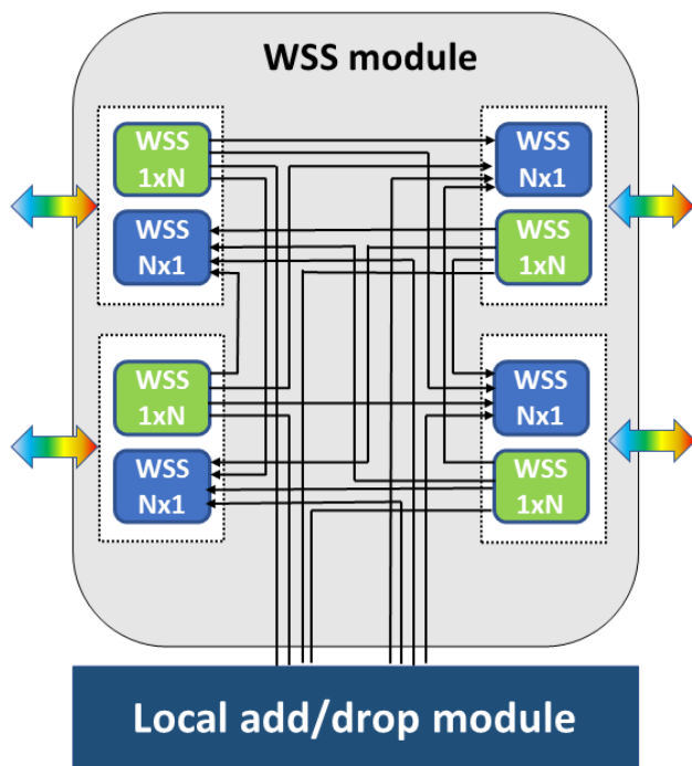
Fig. 1. ROADM architecture enabled by multiple WSS modules.
