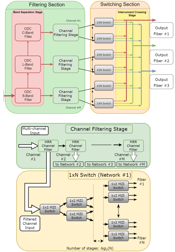
Fig. 2. Circuit model of the proposed WSS structure, highlighting the main operational stages and their block structure.
