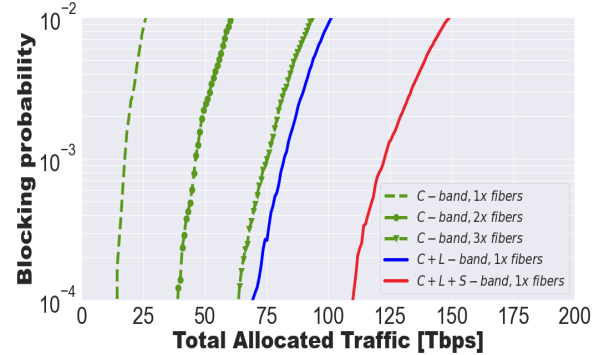
Fig. 13. Blocking probability evaluated over the German network ( \approx 4 THz/band) considering 800G transceivers.
