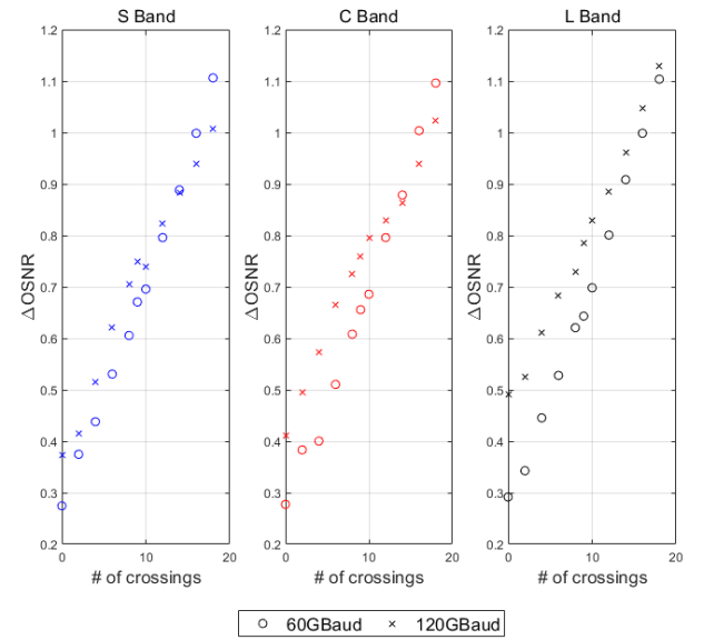
Fig. 7. \Delta\text{OSNR} penalty distribution for tested channel comparing the 60 GBaud and the 120 GBaud performance.
