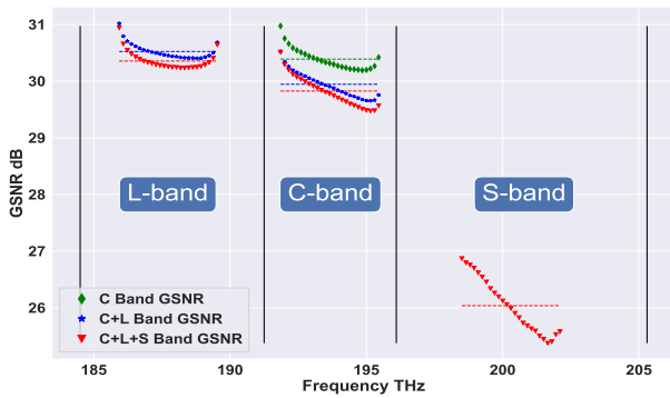
Fig. 8. GSNR vs. frequency for 105 channels (S+C+L-25+40+40 channels) for all scenarios (C-band only, C+L and S+C+L).
