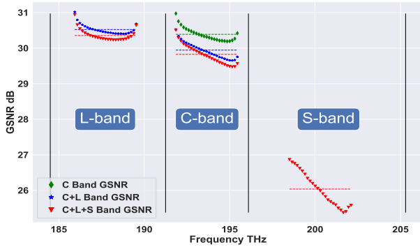
Fig. 8. GSNR vs. frequency for 105 channels (S+C+L-25+40+40 channels) for all scenarios (C-band only, C+L and S+C+L).
