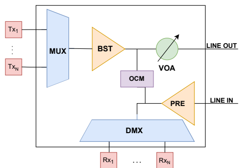
Fig. 1: White-box ROADM architecture.
