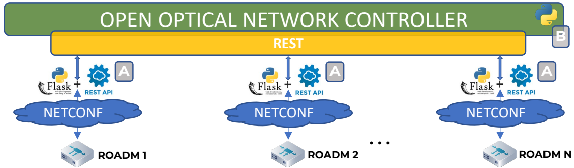
Fig. 2: Conceptual sketch of the software framework: (A) ROADM NETCONF agent; (B) open optical network controller.
