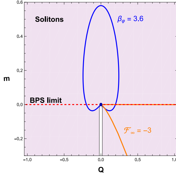
Figure 4.1.1: Parameter space (m, Q) of the background (4.1.9). The blue line represents backgrounds with the same \beta_\phi . In orange, there are backgrounds which agree on the values of circulation at infinity \mathcal{F}_\infty . The dashed red line represents the BPS configurations. The purple region indicates where the solution exists in contrast with the semi-infinite line Q = 0, m < 0 .
