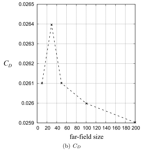
Figure 17: Convergence analysis on aerodynamic coefficients as a function of the domain extension. Wing with AR = 3 .
