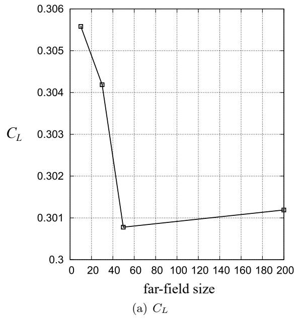
Figure 17: Convergence analysis on aerodynamic coefficients as a function of the domain extension. Wing with AR = 3 .
