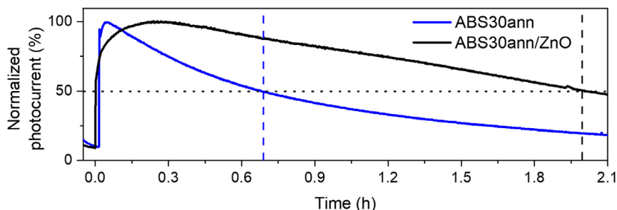
FIGURE 8 | Operational long-term PEC stability test at 1.23 V versus RHE under light exposure of ABS30ann with and without the ALD deposited ZnO protective layer.
