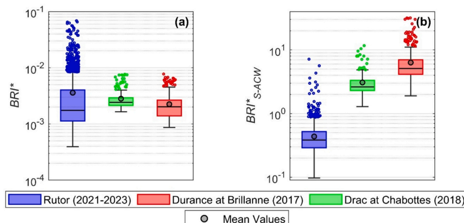
Fig. 13. Box plots comparing BRI^* and BRI^*_{S-ACW} for the Rutor dataset (2021–2023), Durance river at Brillanne (2017) and Drac river at Chabottes (2018).
