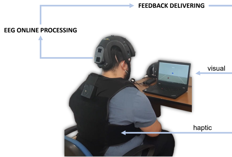
Figure 1. A subject using the proposed BCI system with neurofeedback in extended reality. The system involves EEG acquisition with the Helmate device, online processing, and actuators for visual-haptic feedback delivering.
