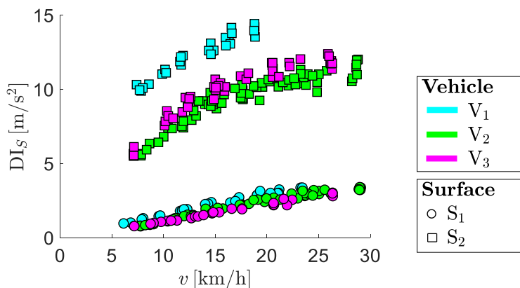
Figure 8. Discomfort index evaluated at the hand-steering interface for the three vehicles on asphalt and pavé surfaces for different vehicle velocities.
