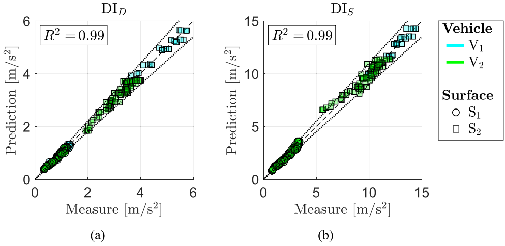
Figure 10. Predicted versus measured discomfort index evaluated at the foot-deck (a) and hand-steering (b) interfaces for V_1 and V_2 on asphalt and pavé surfaces.
