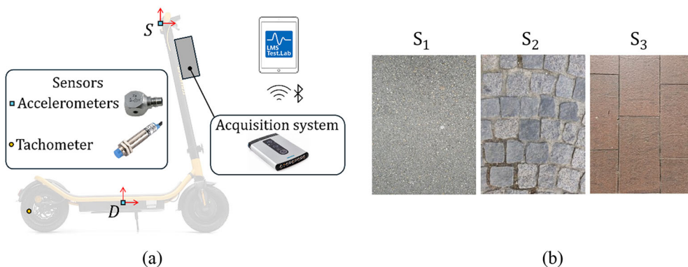
Figure 5. Layout of the experimental instrumentation (a) and road surfaces employed during the on-road tests (b).
