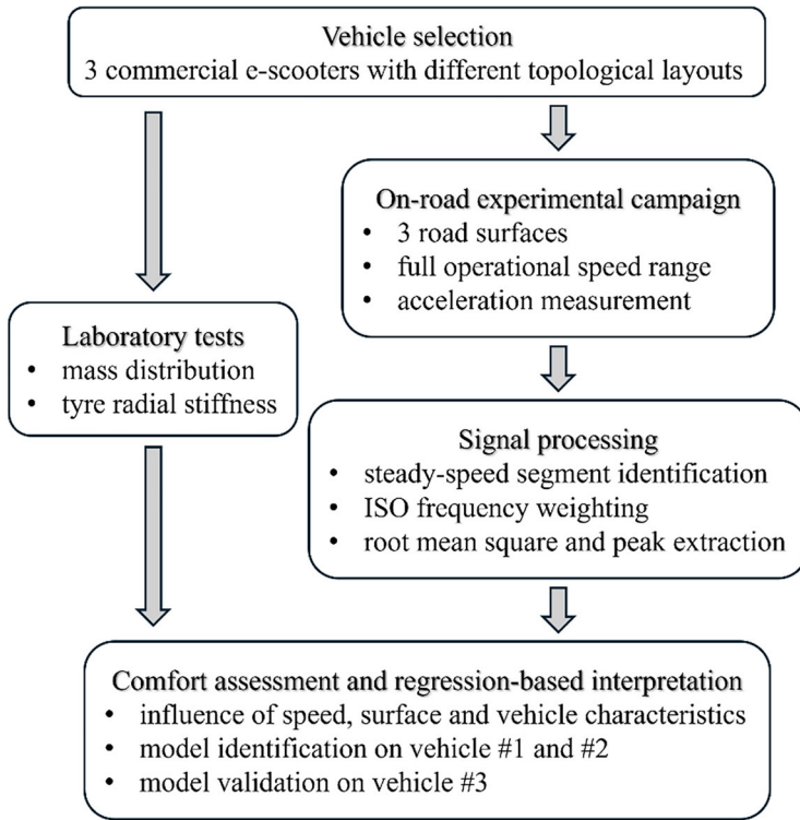
Figure 1. Overview of the proposed framework for e-scooter ride comfort assessment, linking vehicle characterisation, on-road vibration measurements, ISO-based signal processing and regression-based interpretation.
