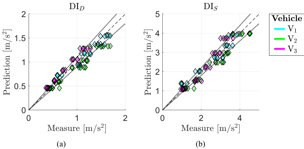
Figure 12. Predicted versus measured discomfort index evaluated at the foot-deck (a) and hand-steering (b) interfaces for the three vehicles on the bike path.
