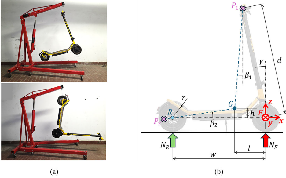
Figure 3. Centre of mass identification through the suspension method: experimental configuration (a) and schematic representation of the methodology employed to determine G coordinates (b).
