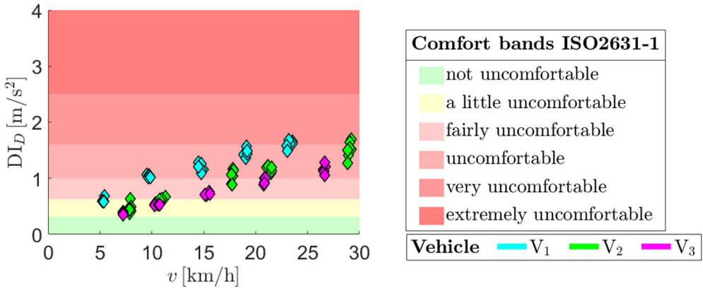
Figure A1. Discomfort index evaluated at the foot-deck interface for the three vehicles on the bike path for different vehicle velocities.
