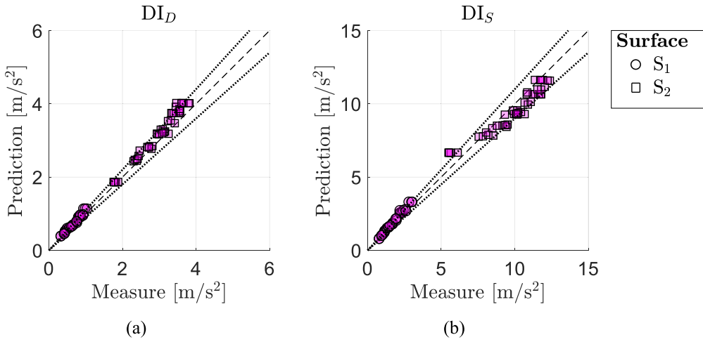
Figure 11. Predicted versus measured discomfort index evaluated at the foot-deck (a) and hand-steering (b) interfaces for V_3 on asphalt and pavé surfaces.
