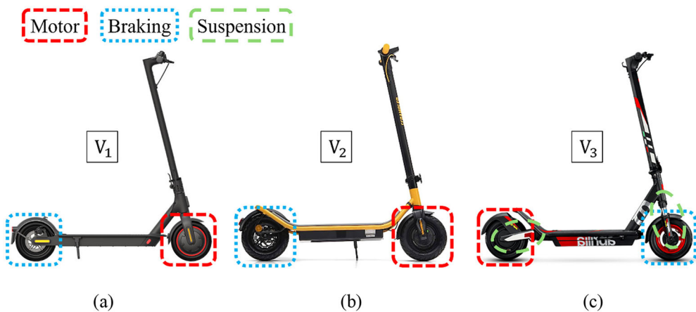
Figure 2. E-scooters analysed in this study with their key layout differences: (a) V_1 , (b) V_2 , and (c) V_3 .
