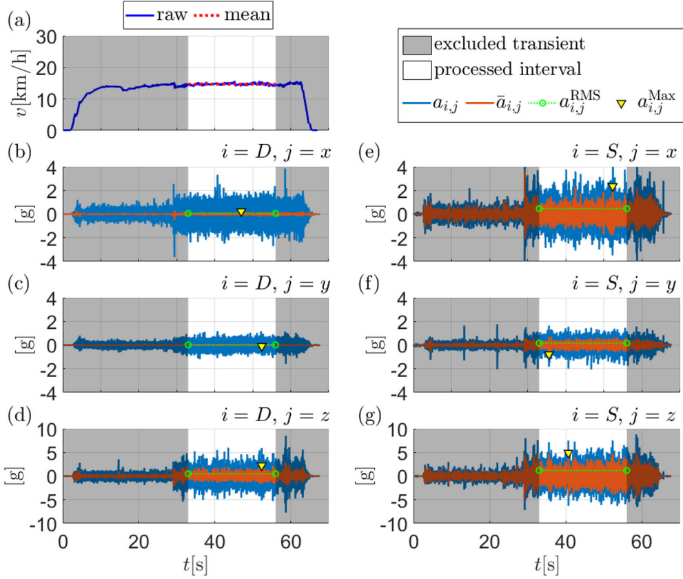
Figure 6. Data processing: vehicle velocity (a), raw and filtered acceleration components measured at the deck (b, c and d) and at the steering (e, f and g), root mean square and maximum values.
