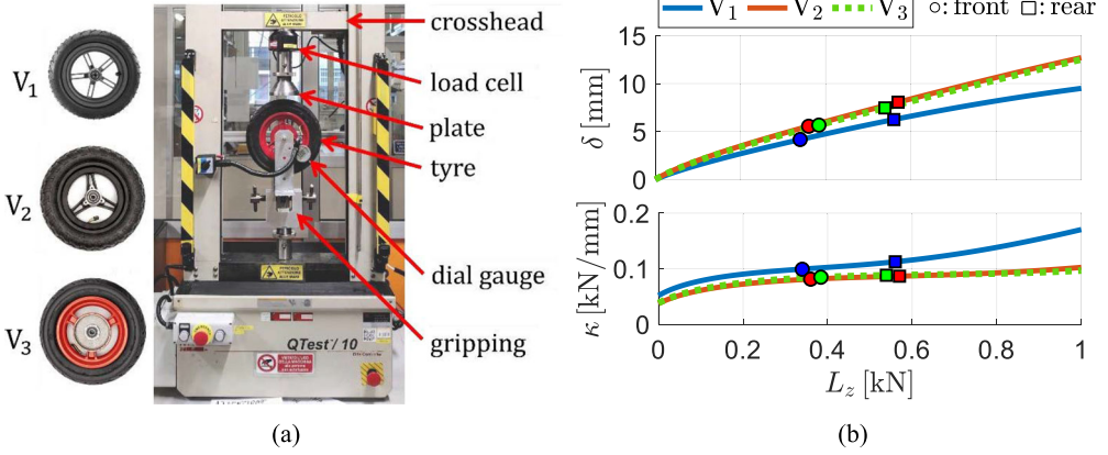
Figure 4. Tyres of the three e-scooters and experimental setup for radial stiffness characterisation (a), tyre deflection and radial stiffness as functions of vertical load (b).
