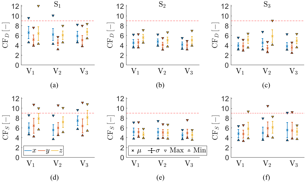
Figure 9. Average, standard deviation, maximum and minimum values of the crest factor evaluated at the foot-deck (a, b, and c) and hand-steering (d, e, and f) interfaces for the three vehicles on asphalt (a and d), pavé (b and e), and bike path (c and f) surfaces.
