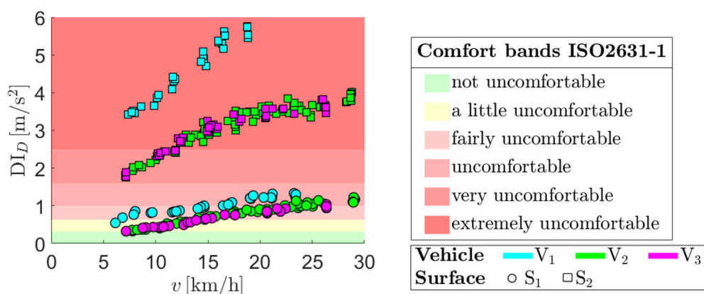
Figure 7. Discomfort index evaluated at the foot-deck interface for the three vehicles on asphalt and pavé surfaces for different vehicle velocities.
