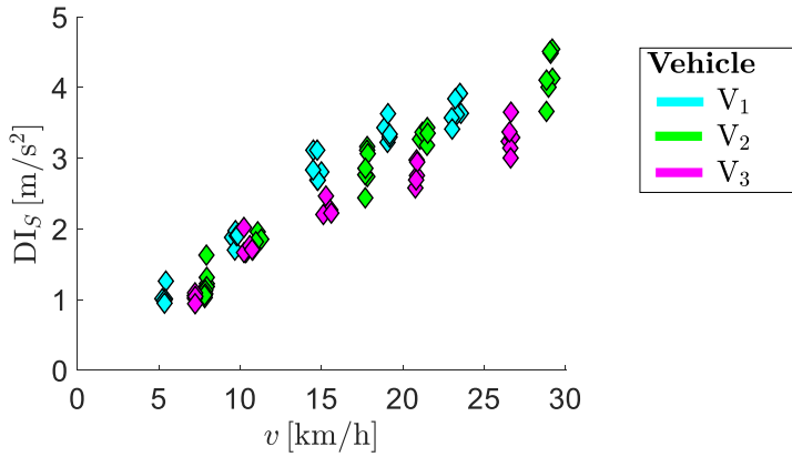
Figure A2. Discomfort index evaluated at the hand-steering interface for the three vehicles on the bike path for different vehicle velocities.
