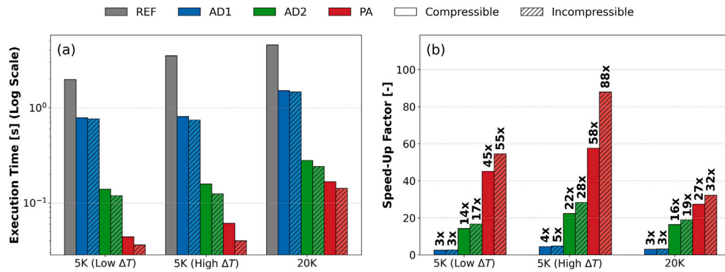
Fig. 8. Comparison of the computational performance of the investigated models: (a) execution time of the core solver on a logarithmic scale; (b) speed-up factor relative to the reference (REF) model.
