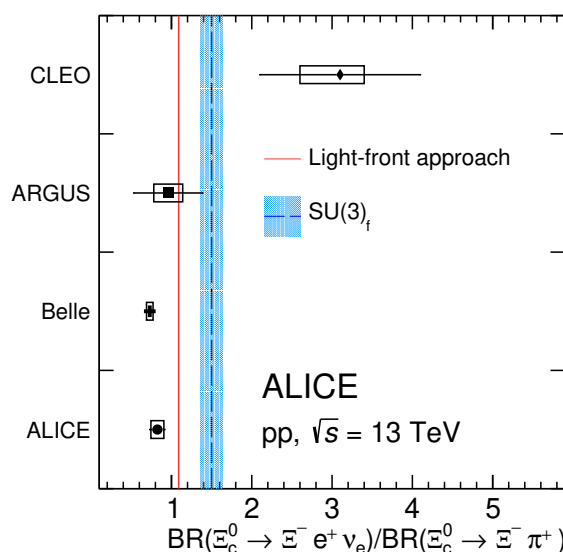
Figure 6. Comparison of \text{BR}(\Xi_c^0 \rightarrow \Xi^- e^+ \nu_e) / \text{BR}(\Xi_c^0 \rightarrow \Xi^- \pi^+) between experiments [58–60] and model predictions [61, 62].
