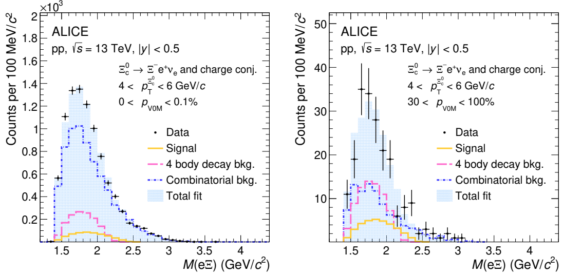
Figure 2. Invariant-mass distribution of e\Xi pairs for \Xi_c^0 \rightarrow \Xi^- e^+ \nu_e in 4 < p_T < 6 GeV/ c , in the high- (left) and low- (right) multiplicity classes. The blue filled distribution shows the total fit and the coloured lines indicate the different sources contributing to the fit.
