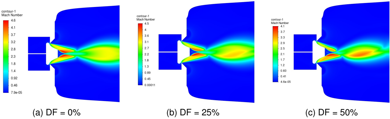
Figure 4 – Mach contours at NPR = 50 for different DF-values
