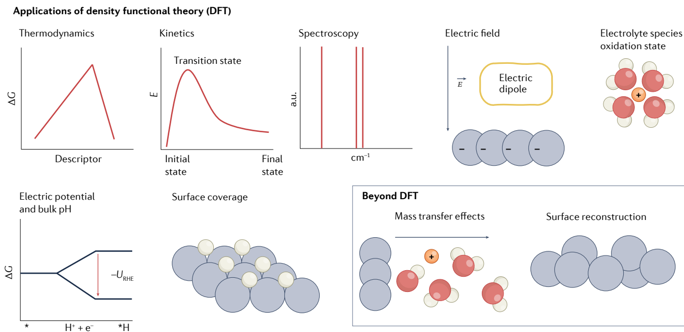
Q31 Fig. 6 | Density functional theory modelling for water electrolysis. Potential and limitations of state-of-the-art density functional theory (DFT) modelling for water electrolysis. RHE, reversible hydrogen electrode.
