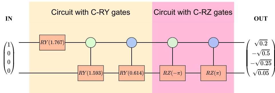
FIGURE 5 | Representation of a Mottonen State Preparation circuit that encodes the state vector [\sqrt{0.2}, -\sqrt{0.5}, -\sqrt{0.25}, \sqrt{0.05}] . The controlled gates, whose circles are colored in green, are active when the control qubit is in state |0\rangle ; otherwise, they are active when the control is in state |1\rangle .
