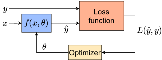
FIGURE 2 | Graphical scheme of the training processing adopted for classification purposes. The model (i.e., the blue rectangle) receives the input data x and estimates the output class they belong to, \hat{y} . The loss function then uses this information to evaluate the difference with respect to the correct target y , generating the magnitude of the error made by the model, L(\hat{y}, y) . Finally, the optimizer closes the loop by considering the actual error and adjusting the parameters \theta of the model to increase its prediction performance during the next iteration.
