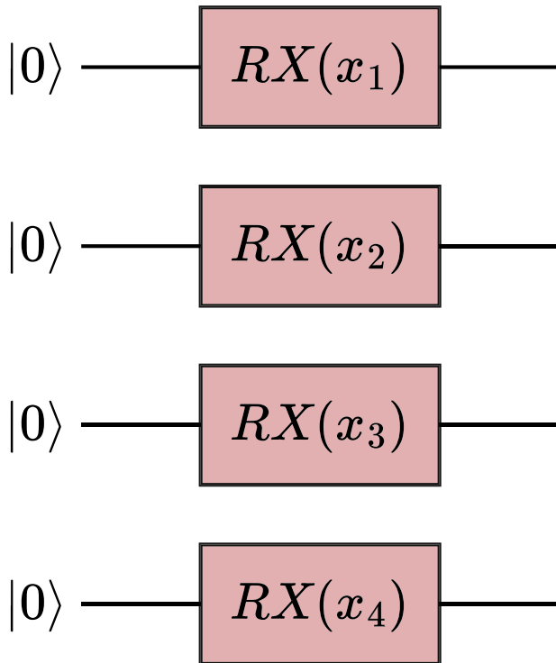
FIGURE 6 | Representation of an Angle encoding strategy using RX as the rotational gate. Each feature of the input vector is embedded in a qubit of the quantum circuit.
