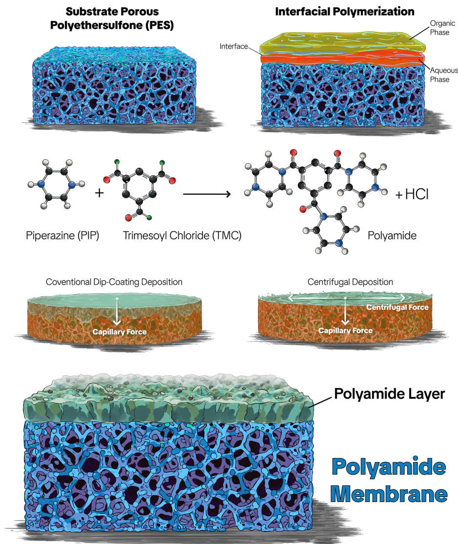
Fig. 7 | Fabrication process for a polyamide thin-film composite (TFC) membrane. A Polyethersulfone (PES) substrate is first coated with an aqueous piperazine (PIP) solution, followed by contact with an organic phase containing trimesoyl chloride (TMC) at the interface, where interfacial polymerization occurs. The reaction between PIP and TMC forms a crosslinked polyamide network with HCl as a byproduct, resulting in the formation of a polyamide selective layer at the top of the PES support. Moreover, a schematic illustration of the CTFD process is compared with conventional dip-coating. In CTFD, centrifugal acceleration drives radial spreading and rapid excess-liquid removal, promoting uniform lateral coverage and more controlled interfacial polymerization.
