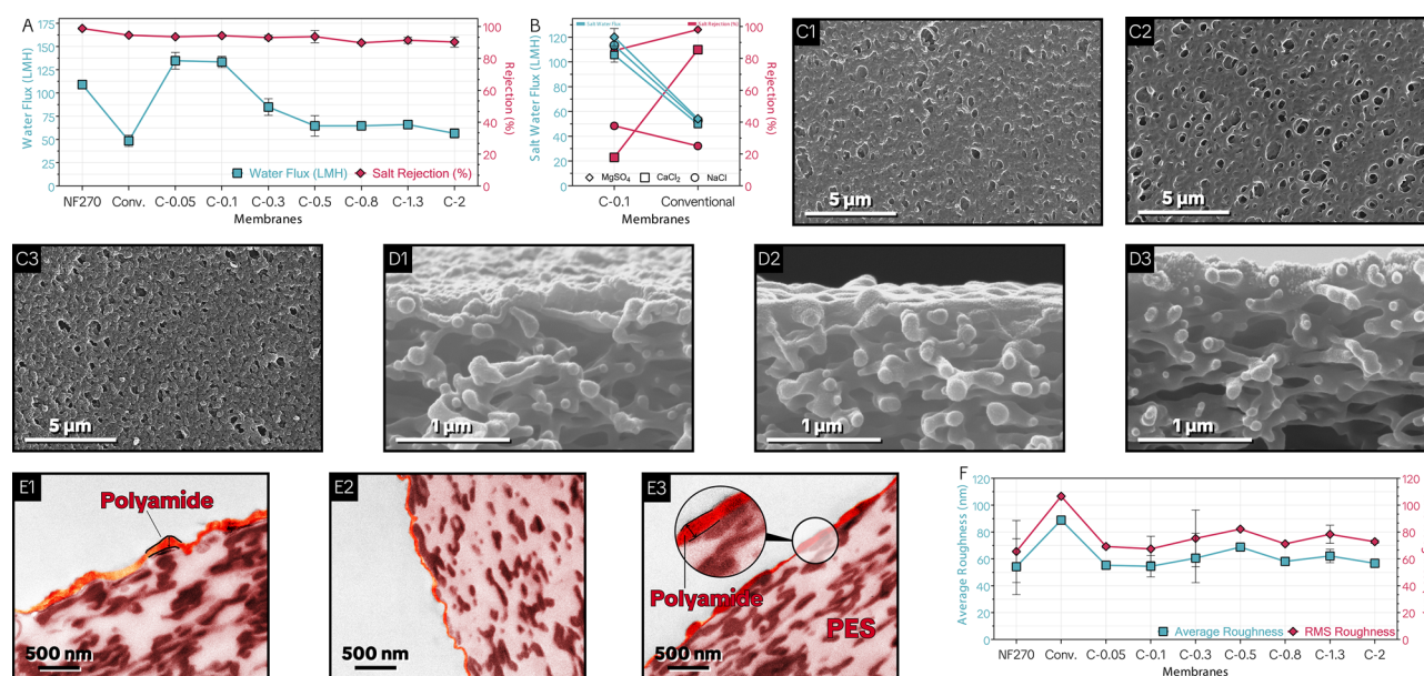
Fig. 5 | Filtration performance and structural analysis of membranes fabricated under a centrifugal force of 3.198 \text{ kg m/s}^2 with varying piperazine (PIP) concentrations. A Water flux and \text{Na}_2\text{SO}_4 rejection for all membranes. B Salt water flux and rejection for other salts ( \text{MgSO}_4 , \text{CaCl}_2 , and \text{NaCl} ) were evaluated only for the conventional membrane and the optimized CTFD membrane (C-0.1). C 1 – C 3 Top-view FESEM images for the conventional, C-0.1, and C-2 membranes, respectively, showing smoother, less textured surfaces at lower PIP loadings (e.g., 0.1 wt.%) and
