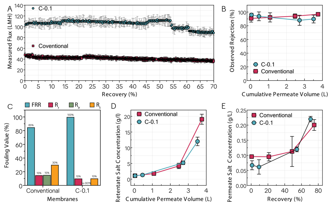
Fig. 6 | High-recovery and fouling performance of the conventional and CTFD membranes. A, B, D, E High-recovery open-loop cross-flow filtration performance of conventional and CTFD membranes using Na 2 SO 4 feed solution. A Measured flux as a function of recovery, showing the higher and more stable flux of the CTFD membrane compared to the conventional one. B Observed rejection as a function of cumulative permeate volume, where the conventional membrane exhibits a gradual increase in rejection while the CTFD membrane shows minor variability.
