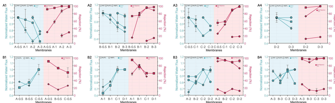
Fig. 3 | Dead-end filtration performance of TFC membranes under varying fabrication parameters. A 1 –A 4 Normalized water flux and salt rejection for Na 2 SO 4 , MgSO 4 , and NaCl as a function of piperazine (PIP) concentration at fixed centrifugal forces. B 1 –B 4 Normalized water flux and salt rejection for Na 2 SO 4 ,
