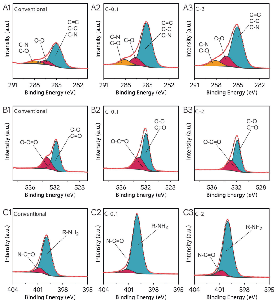
Fig. 4 | Surface chemistry analysis of the conventional, C-0.1, and C-2 membranes, respectively. Deconvoluted high-resolution XPS spectra of (A 1 –A 3 ) C 1 s, (B 1 –B 3 ) O 1 s, and (C 1 –C 3 ) N 1 s show the characteristic chemical bonding associated with amide formation.
