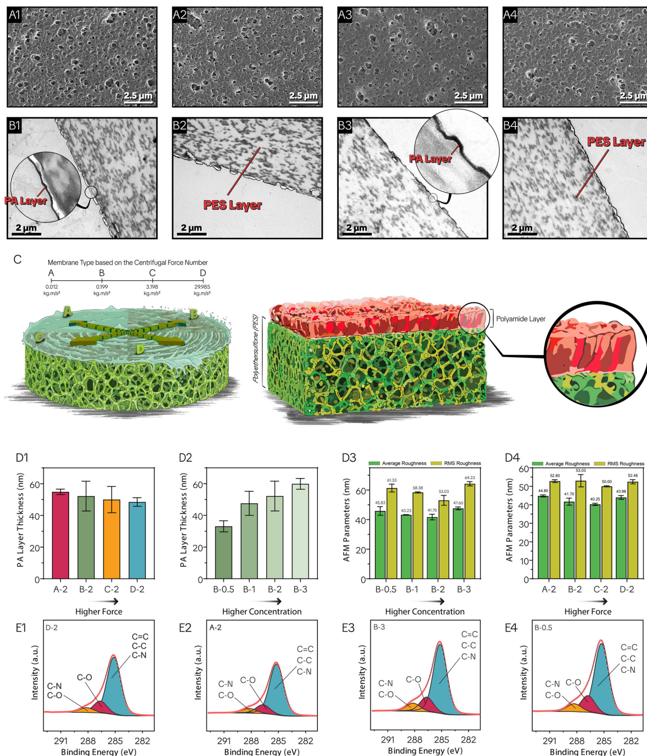
Fig. 1 | Morphological, topographical, and surface chemical characterization of polyamide membranes fabricated with varying piperazine (PIP) concentrations and centrifugal forces (B-0.5, B-3, A-2, and D-2). A 1 –A 4 Top-view FESEM images showing textured morphology of diffusion-limited interfacial polymerization (IP). B 1 –B 4 Cross-sectional TEM images illustrating the formation of thin polyamide selective layers across all CTFD membranes. Thicker layers appeared at higher PIP concentrations, while higher centrifugal forces yielded slightly thinner films. C Schematic illustration of the PES substrate showing the application of various centrifugal forces during deposition and the formation of the polyamide selective
