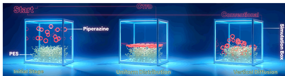
Fig. 2 | Molecular dynamics simulation. Final distribution of piperazine (PIP) monomers on the polyethersulfone (PES) substrate after molecular dynamic simulation for CTFD and conventional techniques. The centrifugal deposition configuration appeared to promote enhanced monomer uniformity and surface coverage compared to the disordered distribution observed in the conventional approach.
