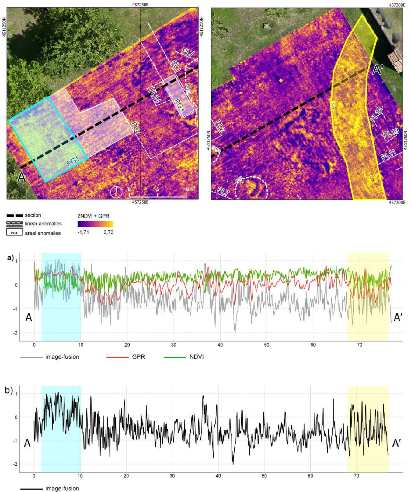
FIGURE 19 | Examples of anomalies detected in the enhanced map, represented in different shades of orange-yellow: left, an anomaly previously detected by spectral index maps, highlighted in light blue; right, an anomaly previously detected by spectral index maps, RGB orthophoto and GPR data, highlighted in yellow. (a) Diagram of comparison between the DN of the three calculated maps: enhanced map, GPR slice (30cm) and NDVI spectral index; (b) a diagram plotting only the DN on the raster cross-correlation map section A–A'.
