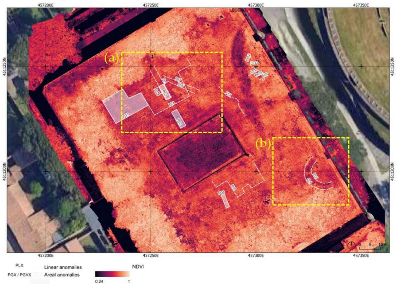
FIGURE 5 | Detected spectral anomalies—in white—overlapped on the normalized difference vegetation index map. Yellow rectangles (a), (b) indicate areas corresponding to zoomed-in images of specific anomalies.
