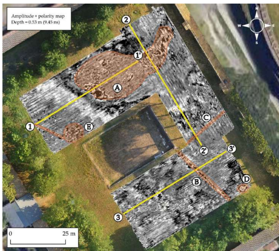
FIGURE 11 | Kirchhoff migration time-slice at 0.53 m b.g.l. (9.45 ns corrected return time). Notable anomalies are highlighted in orange, whereas B-scan sections 1–1', 2–2' and 3–3' are marked in yellow.
