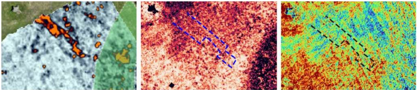
FIGURE 15 | Zoomed-in Area C, illustrating the different detection responses of GPR, NDVI and RN index to the same anomaly, underscoring the methodological variation in anomaly identification.
