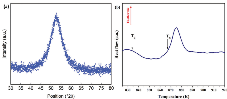
Figure 3. \text{Co}_{66}\text{Fe}_4\text{Mo}_2\text{Si}_{16}\text{B}_{12} metallic glass microfibers are characterized by a) XRD analysis b) DSC measurement.
