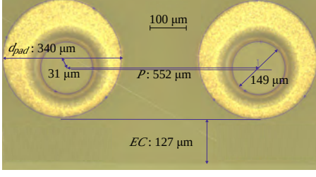
Fig. 18. Microscope image: Dimensional measurement of the prototype.
