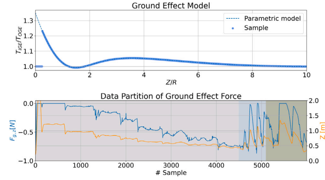
Fig. 5. Data set of simulated flight corrupted with ground effect. Top: Parametric model of quadrotor ground effect [33] (x-axis represents the ratio between altitude above the ground, Z , and propeller radius, R , and y-axis represents the ratio between the lift experienced while hovering IGE and OGE) and data samples collected from our implementation in the simulator. Bottom: Collected flight data for training: blue curve indicates ground effect force along body z -axis, F_{IGE} , orange curve indicates the altitude above the ground of the quadrotor, and shaded areas represent data partition into training/validation/test data set. (For interpretation of the references to color in this figure legend, the reader is referred to the web version of this article.)
