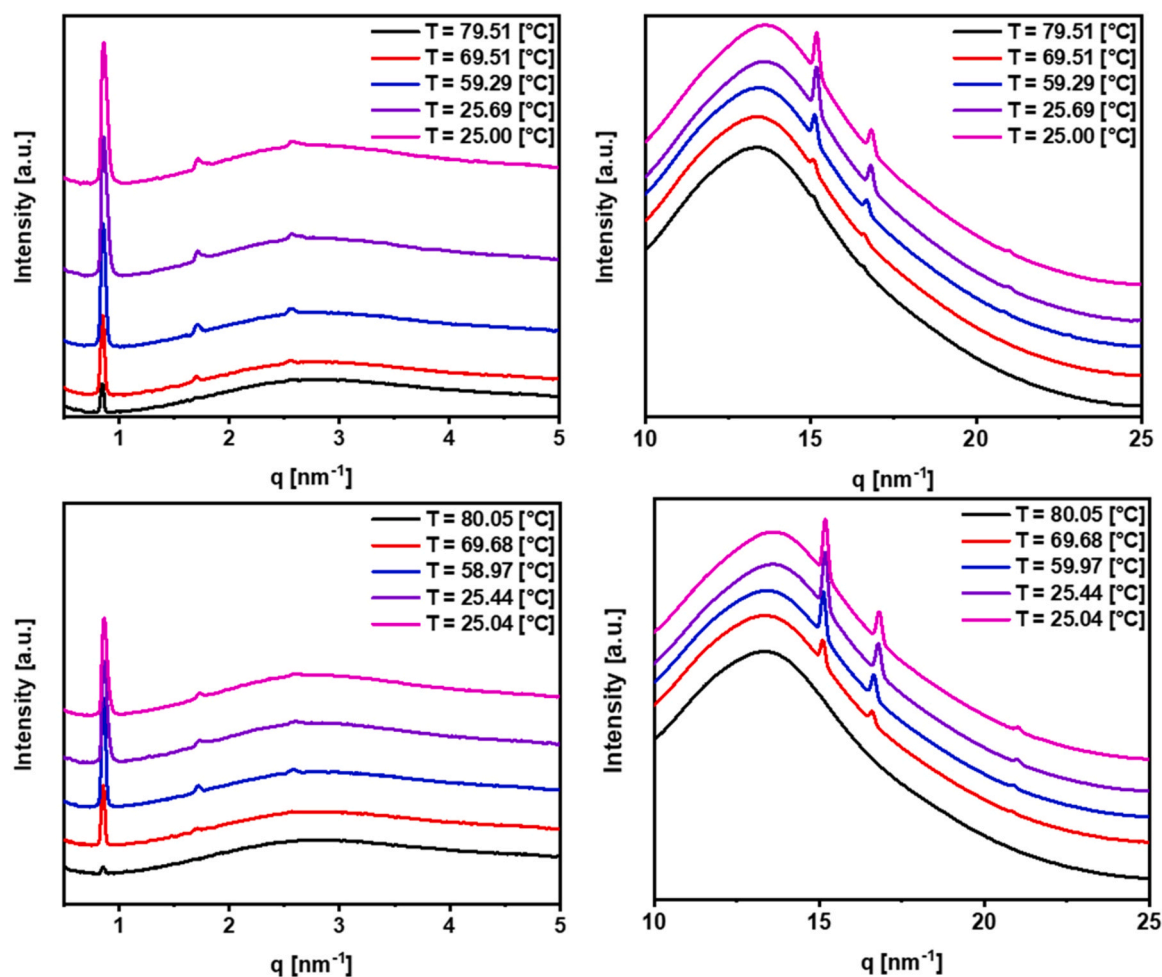
Fig. 8. SAXS (left side) and WAXS (right side) diffractograms of the 5%wt RBXP/SO oleogel. Comparison between data recorded without (top part) and with (bottom part) constant shear rate ( \gamma = 1000 \text{ s}^{-1} ) applied.
