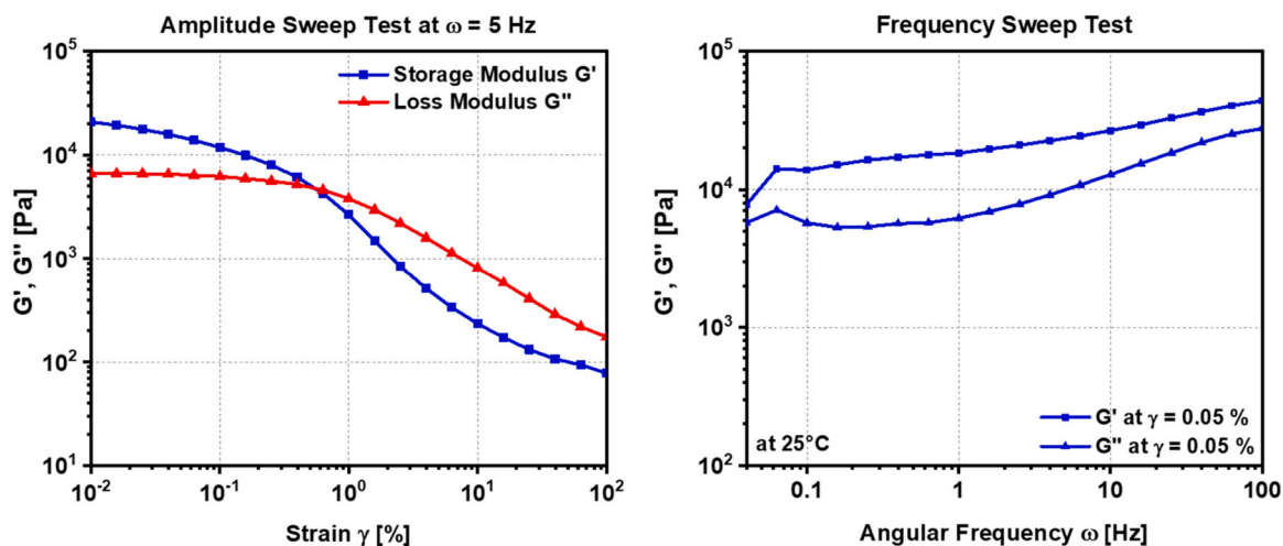
Fig. 10. Amplitude Sweep test results investigated at 5 Hz fixed frequency (left side); Frequency Sweep test results investigated at 0.05% of fixed strain (right side).
