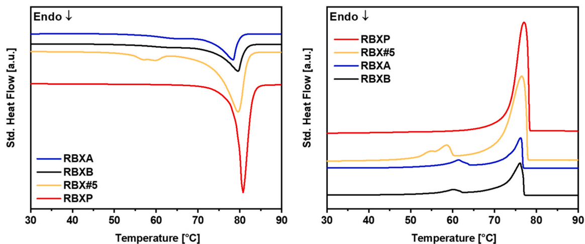
Fig. 6. Melting and crystallisation profiles of RBXs tested as oleogelators.
