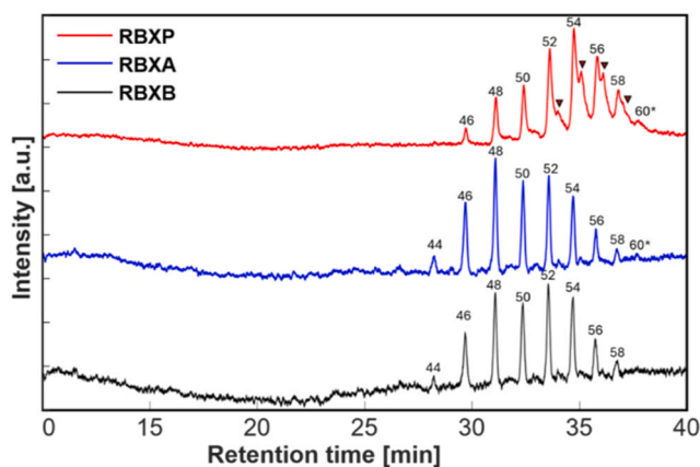
Fig. 1. LC-ELSD chromatograms and relative mass fractions of the wax ester fraction of the laboratory-extracted and commercial RBXs. Error bars represent the standard deviation of n = 3 measurements. *Peak below the limit of quantification.
