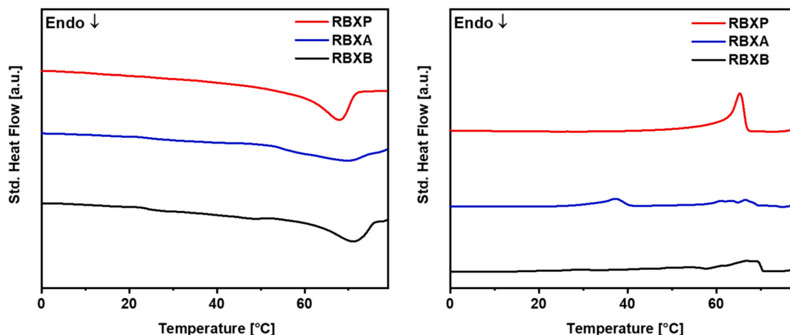
Fig. 7. Melting and crystallisation profiles of 5%wt RBXs/SO.
