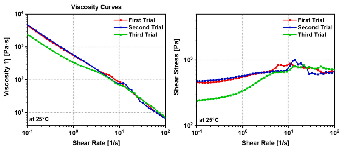
Fig. 12. Viscosity Curves (left side) and Shear Stress Profiles (right side) recorded during the rotational analysis.
