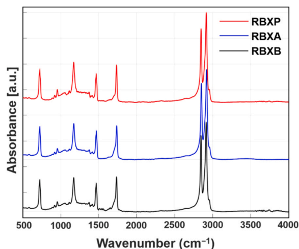
Fig. 2. FTIR spectra collected for the laboratory-extracted and commercial RBXs samples.
