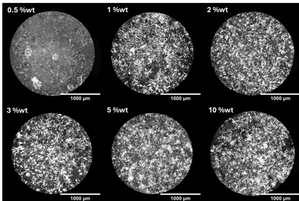
Fig. 3. PLM images of the RBXP/SO oleogels at Different Concentration formed with static cooling conditions, 10x magnification.
