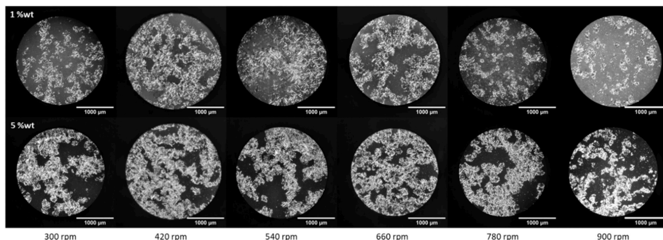
Fig. 4. PLM images of the 1%wt and 5%wt RBXP/SO oleogels at different stirring rates applied, 10x magnification.
