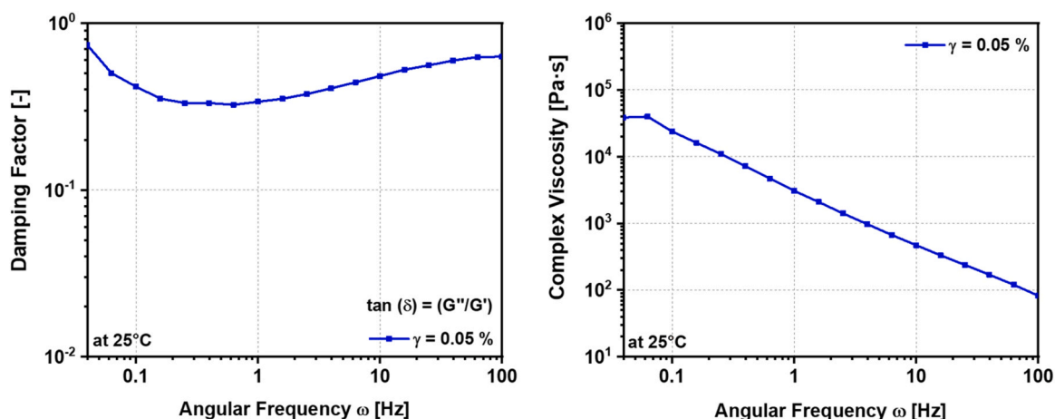
Fig. 11. Damping Factor (left side) and Complex Viscosity (right side) recorded during the Frequency Sweep oscillatory analysis at 0.05% of fixed strain.
