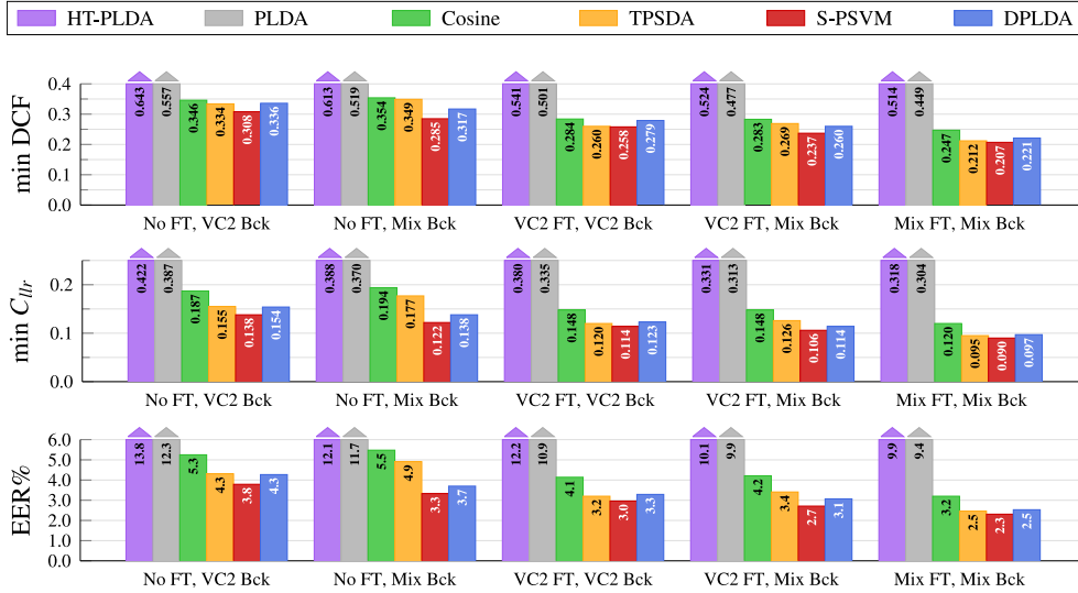
Fig. 1. Minimum DCF, minimum C_{IIr} and EER % for different back-ends with SAM-ResNet-100 front-ends, without fine-tuning (No FT), fine-tuned with VC2 (VC2 FT), and with CTS + VC2 (Mix FT) data. As back-ends we consider both models trained with VC2 (VC2 Bck) and CTS + VC2 (Mix Bck) data.
