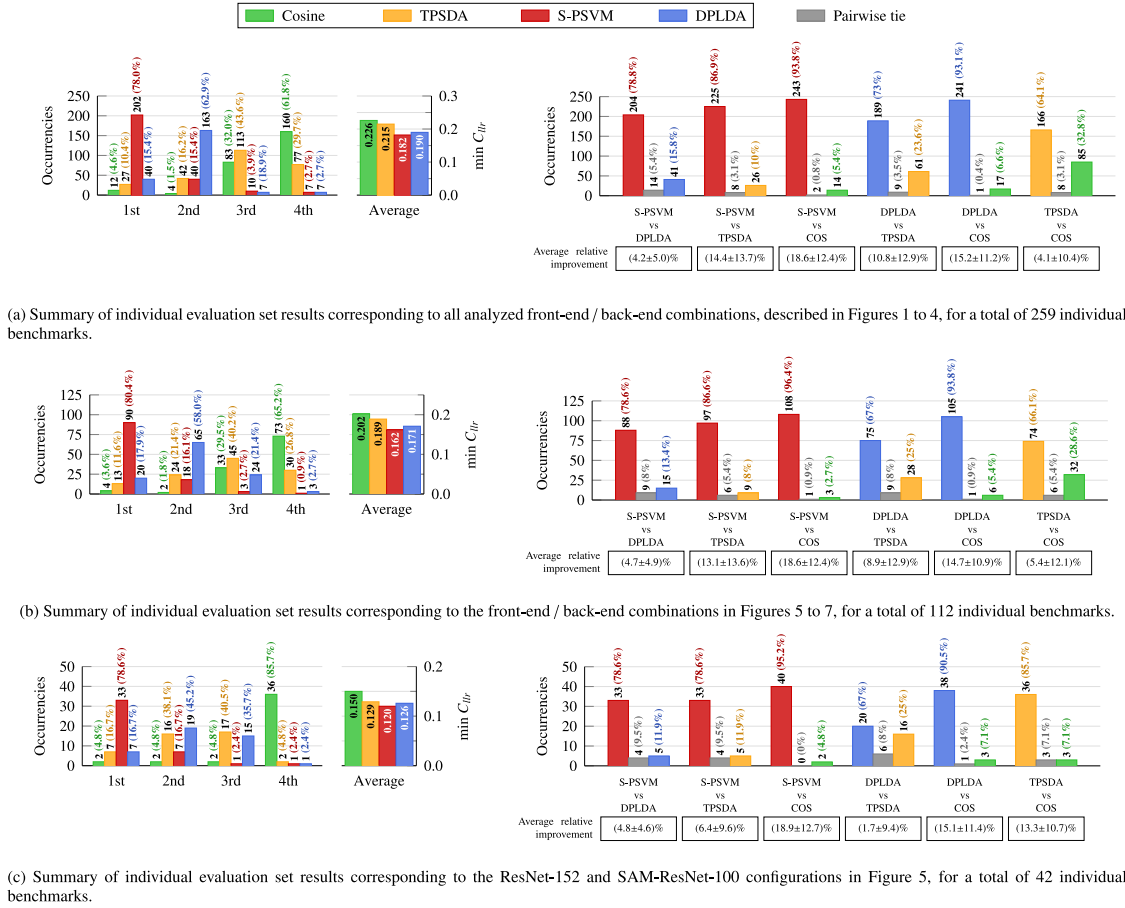
Fig. 15. Summaries of relative back-end rankings for cosine, TPSDA, S-PSVM and DPLDA on individual evaluation sets, and corresponding global geometrical average minimum C_{llr} . Left: number and percentage of times each back-end achieves a given rank. In case of ties (same result up to the third decimal digit) we assign the same rank to both back-ends (thus the total number of back-ends achieving a given rank may differ from the total number of considered benchmarks). Right: Pairwise comparisons. For each back-end pair we report how many times each model achieves better results, and the number of ties. The best performing classifier is on the left of each group. Below each group we report the average improvement, measured as the arithmetic mean of all relative improvements, computed on each evaluation set for each front-end/back-end combination, of the best performing back-end over the worst one, and the corresponding standard deviation.
