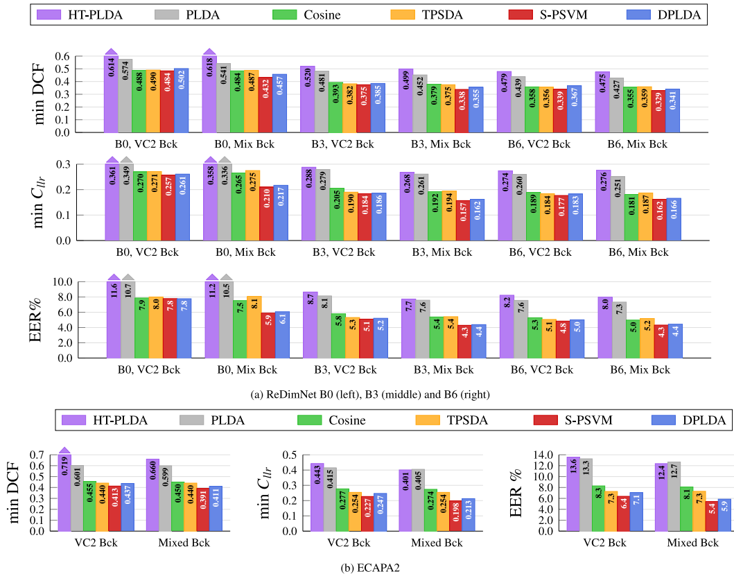
Fig. 4. Minimum DCF, minimum C_{ltr} and EER % for different back-ends with off-the-shelf front-ends. For each back-end, we consider both models trained with VC2 (VC2 Bck) and Mixed CTS + VC2 (Mix Bck) data.
