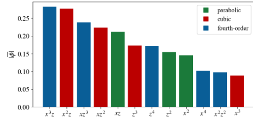
Figure 5: Generalized variables beeswarm plot for the [0^\circ/90^\circ/0^\circ] laminated beam with L/h=10
