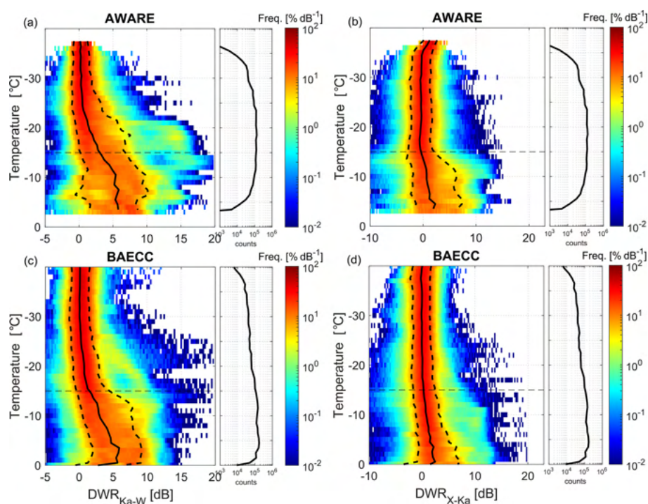
Figure 1. Density plots of DWR_{Ka,W} (a, c) and DWR_{X,Ka} (b, d) as a function of temperature for AWARE (a, b) and BAEC (c, d) datasets. The dashed lines indicate the 10th and 90th percentiles. The subplots on the right of each panel indicate the number of samples per temperature level.
