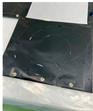
Figure 1. MLI blankets with integrated FBG sensors.
