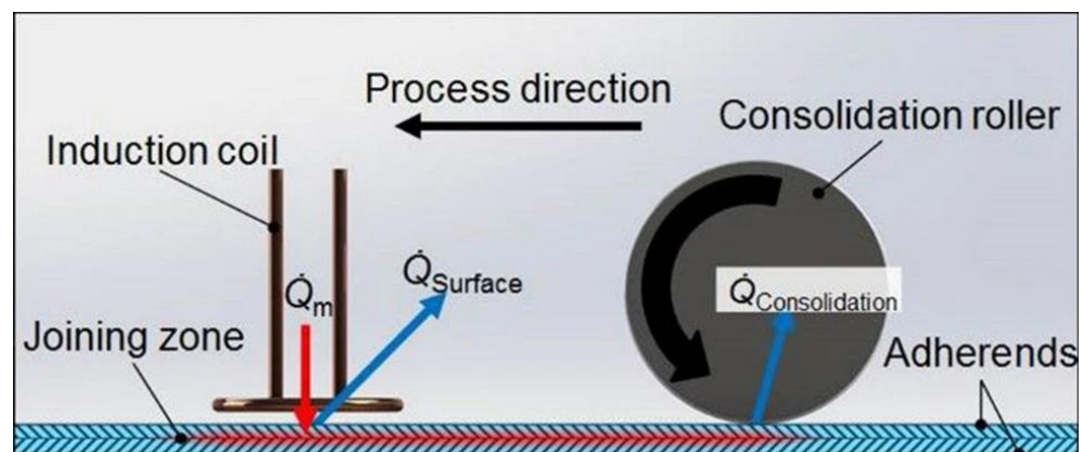
Figure 8. The three key heat fluxes that affect the continuous induction heating-assisted welding process. \dot{Q}_m is the heat input resulting from the induction coil, \dot{Q}_{\text{surface}} is the heat removed from surface cooling, and \dot{Q}_{\text{consolidation}} is the heat removed by conduction through the consolidation roller. Reprinted from [34] under Creative Commons CC BY License.
