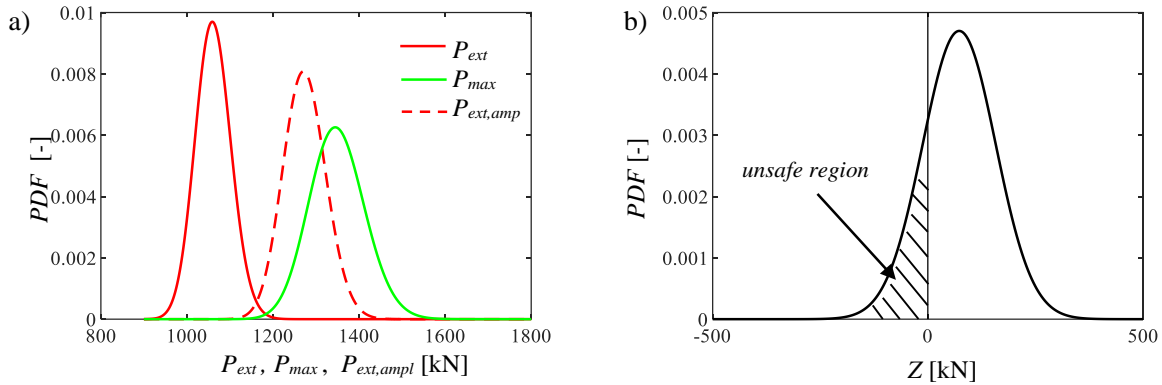
Fig. 9 Computation of the failure probability: a) comparison between the probability density functions of both the capacity (i.e., P_{max} ) and demand (i.e., P_{ext} and P_{ext,ampl} ); b) limit state function and unsafe region.
