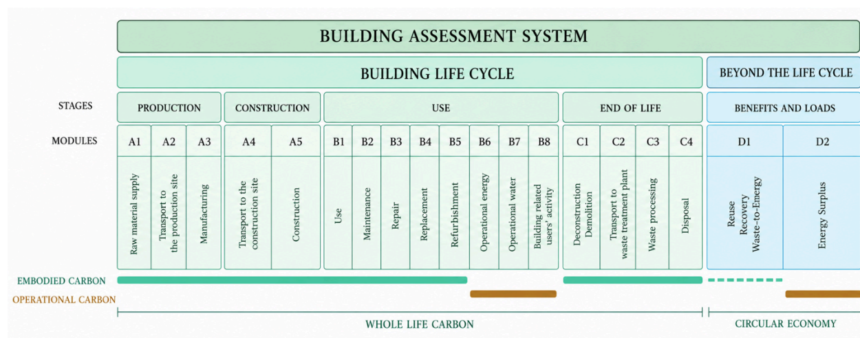
Figure 3: Building assessment framework (Source: Authors' interpretation based on EN 15978:2026).
