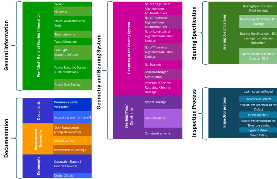
Fig. 1. Database structure.
