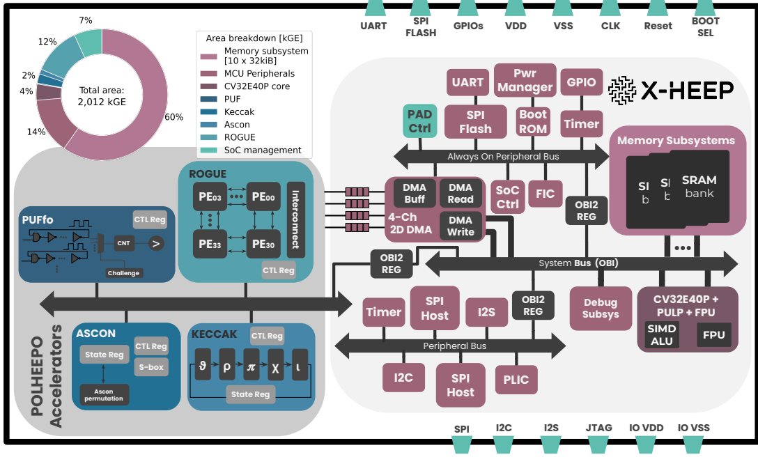
Figure 2: PolHEEPo system overview and post-synthesis area breakdown. Standard X-HEEP components are highlighted in pink, while custom-integrated accelerators are shown in blue, using a consistent color code across both views.
