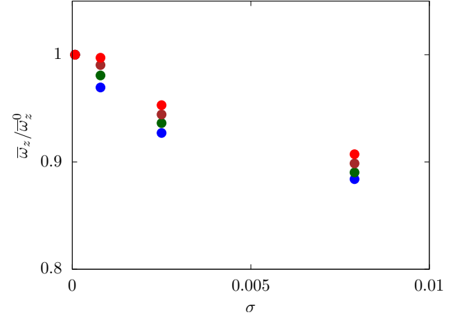
Figure 8: Spanwise component of the particle angular velocity \bar{\omega}_z as a function of the wall permeability \sigma for the different volume fractions considered. The angular velocity is normalized by the value obtained over rigid walls \bar{\omega}_z^0 . The blue, green, brown and red symbols are used to distinguish \Phi = 0.06, 0.12, 0.24 and 0.3 .
