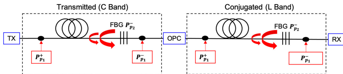
Figure 1. Raman fiber laser amplifier for C and L band with a half-open cavity random lasing designed for a 10 THz OPC-based transmission system.
