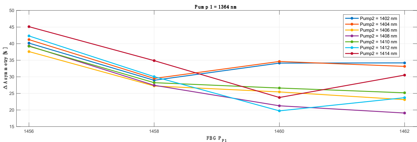
Figure 6. Asymmetry difference between worst and best performing channel in a 50 channels transmission band based on the results shown in Figure 5.
