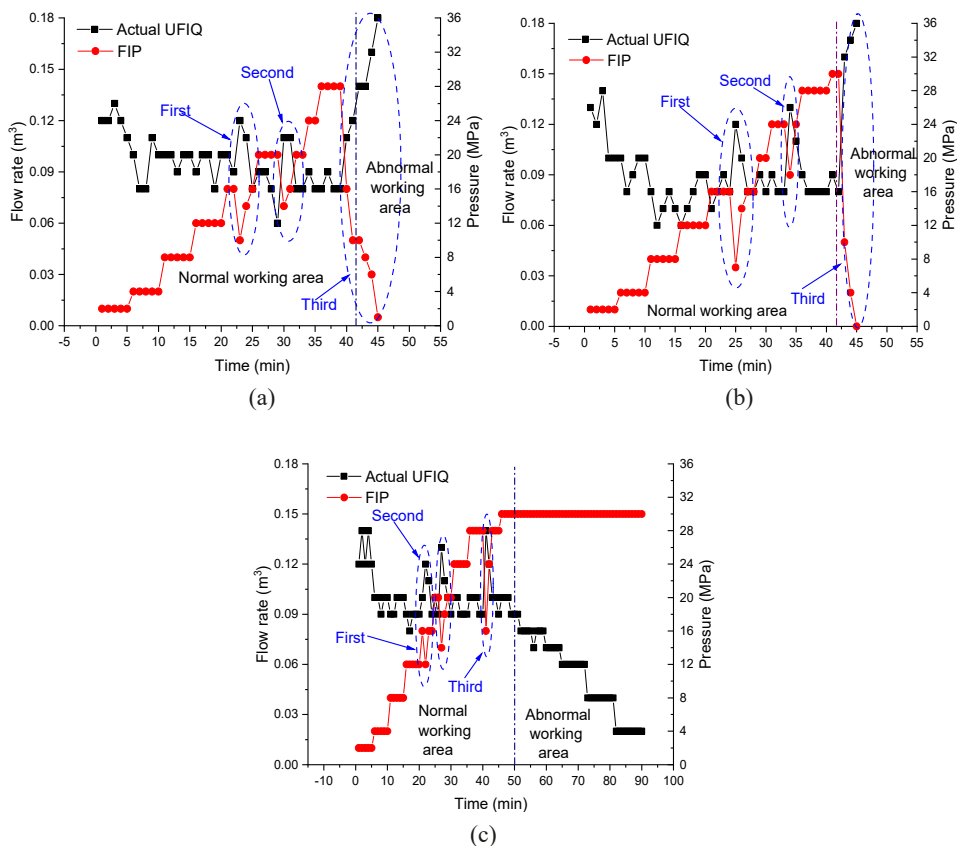
Fig. 13. The change trend diagram of UFIQ and FIP of each fracturing hole in the HF process: (a) 1 # fracturing hole; (b) 2 # fracturing hole; (c) 3 # fracturing hole
