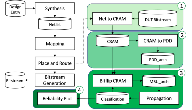
Figure 1: VeriPlace fault simulation flow
