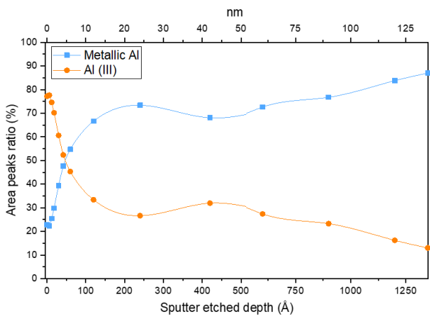
Figure 3: Al narrow scans and related chemical state distribution along sputter depth (with reference to Al_2O_3 calibration) in virgin (a,c) and recycled (b,d) conditions.
