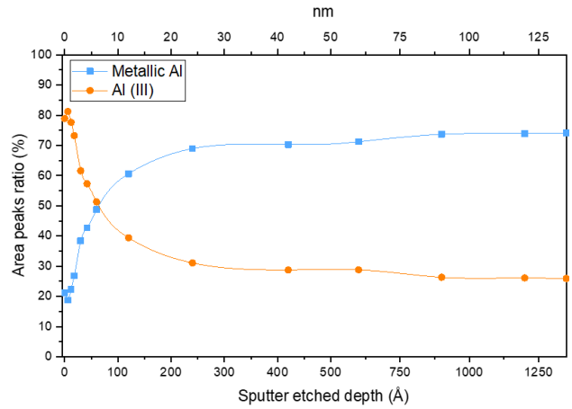
Figure 3: Al narrow scans and related chemical state distribution along sputter depth (with reference to Al_2O_3 calibration) in virgin (a,c) and recycled (b,d) conditions.
