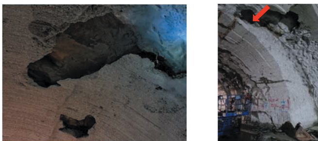
Figure 1. Examples of defects in tunnel lining with reduced thickness, identified during the refurbishment of the Monte Bianco Tunnel in Italy, after milling approximately 25–30 cm of the lining with a roadheader (courtesy of Traforo del Monte Bianco GEIE).
