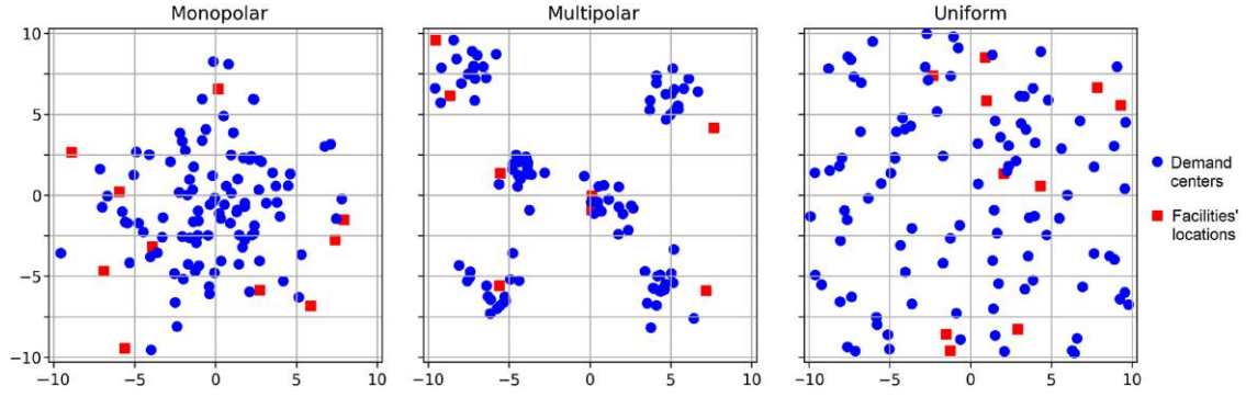
Figure 3. (Color online) Examples of the Different Topologies for 100 Demand Centers and 10 Potential Facilities' Locations
