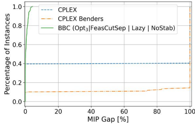
Figure 4. (Color online) Cumulative Percentage of Instances Solved Within the Time Limit Up to Any MIP Gap Percentage for BACOP1
