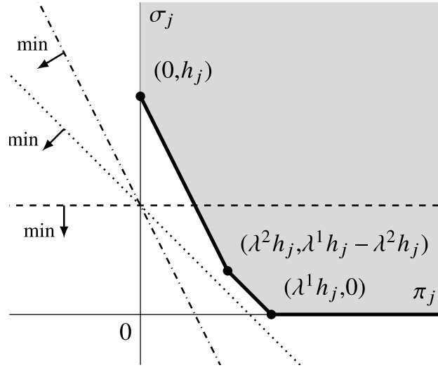
Figure 2. Geometric Representation of Proposition 2
