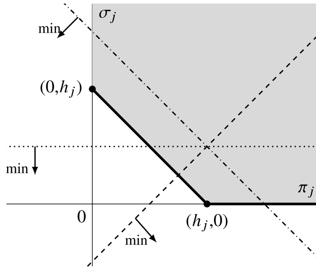
Figure 1. Geometric Representation of Proposition 1
