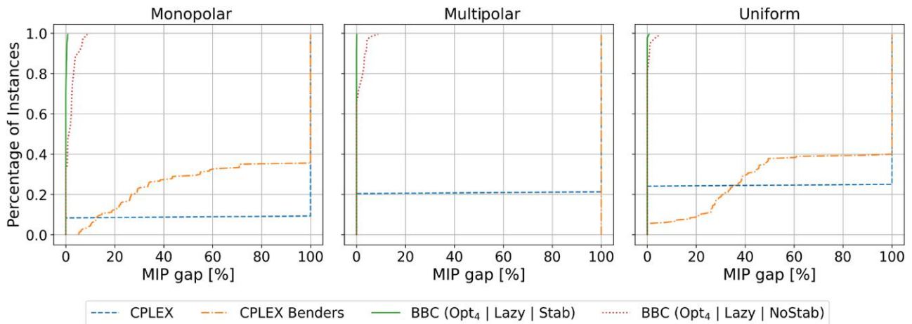
Figure 5. (Color online) Cumulative Percentage of Instances Solved Within the Time Limit Up to Any MIP Gap Percentage for BACOP2
