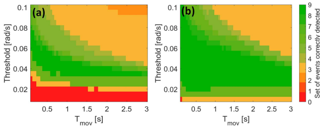
Fig. 11. Detection map considering all T fibers and all realizations of the 3 events (a) with f_s = 48.83 kHz and (b) with f_s = 95.4 Hz.
