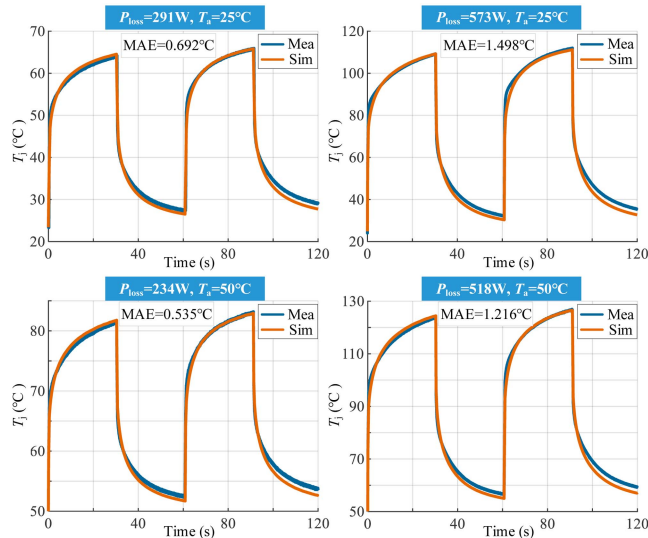
FIGURE 16. Transient simulation and measurement comparison under different boundary conditions and power losses.
