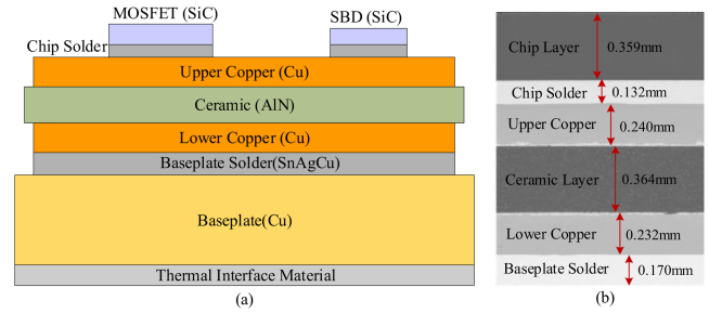
FIGURE 2. Cross-sectional structure of the power module. (a) Notional diagram of the multi-layer layout. (b) Microscopic image.
