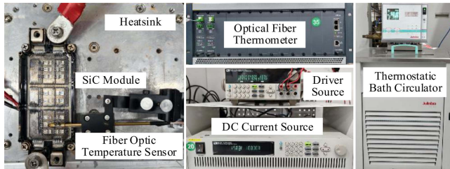
FIGURE 14. Junction temperature test bench for SiC power modules.
