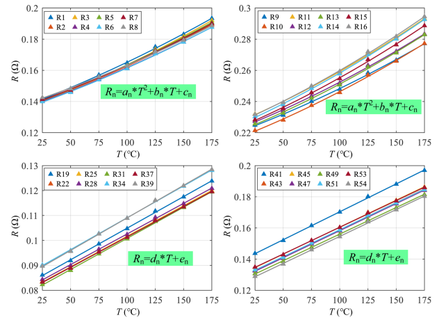
FIGURE 7. Temperature-related thermal resistance fitting results.
