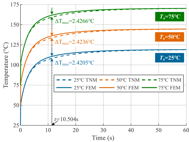
FIGURE 13. Comparison of FEM and TNM under different boundary conditions.
