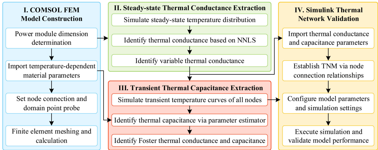
FIGURE 9. Overall TNM modeling process.
