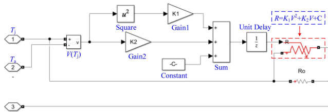
FIGURE 10. Implementation method of variable thermal resistance.
