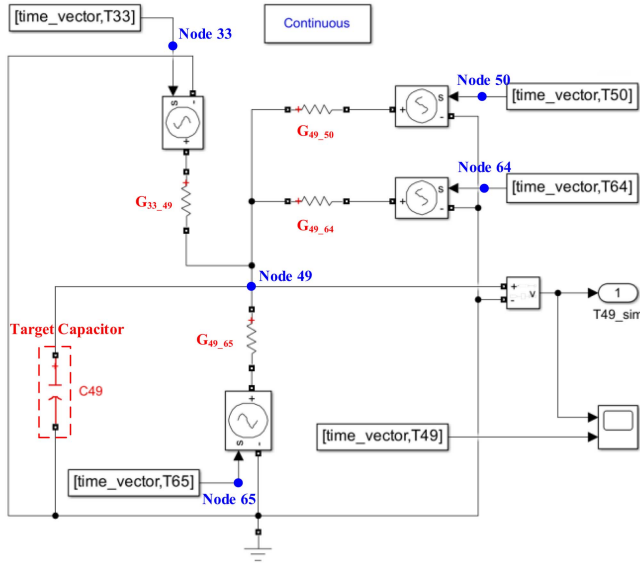
FIGURE 8. Thermal capacitance extraction through local thermal network.
