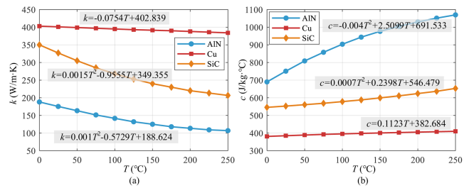
FIGURE 3. Temperature-dependent material properties of the SiC power module. (a) Thermal conductivity. (b) Specific heat capacity.
