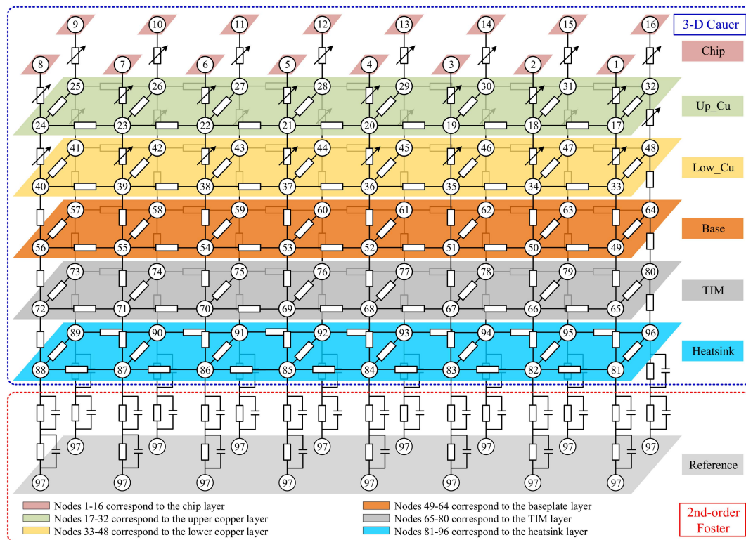
FIGURE 6. Structure of hybrid 3-D temperature-dependent TNM.
