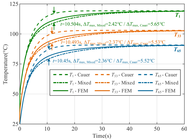
FIGURE 12. Comparison of the proposed model, conventional model, and finite element simulation.
