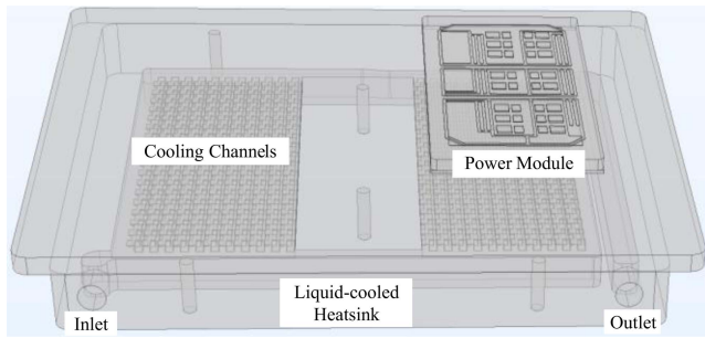
FIGURE 4. COMSOL 3-D model of the module and heatsink.
