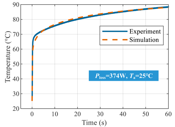
FIGURE 5. Comparison of transient temperature curves between experiment and simulation (max error 2.1%).
