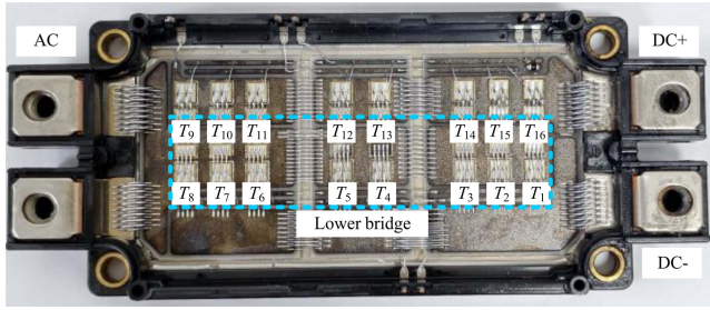
FIGURE 1. Structure of Rohm BSM300D12P2E001.
