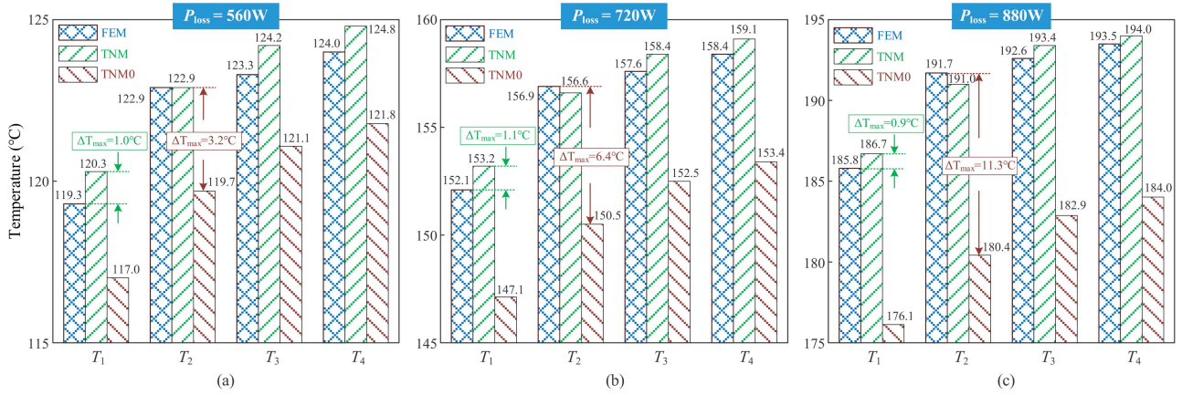
FIGURE 11. Steady-state accuracy validation. (a) 560 W Condition. (b) 720 W Condition. (c) 880 W Condition.
