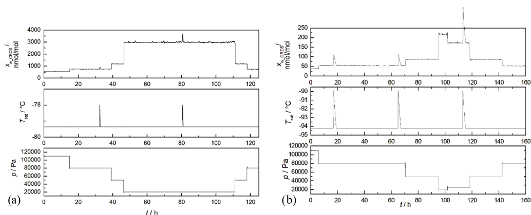
Figure 9. Response of the humidity generator at step changes of the saturation pressure between 1100 and 200 hPa. The saturation temperature has been maintained at a constant value of (a) -80 °C and (b) -95 °C.
