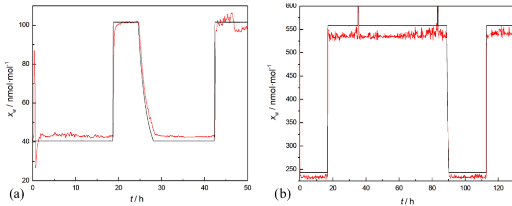
Figure 8. Response of the humidity generator at step changes of the saturation temperature; (a) between -95^\circ\text{C} and -90^\circ\text{C} (that is, between 40 and 100 ppb) and (b) between -85^\circ\text{C} and -80^\circ\text{C} (that is, between 240 ppb and 550 ppb). Measurements have been carried out at 2 \text{ l}\cdot\text{min}^{-1} at a pressure of 1000 hPa. The red line represents the water vapour amount fraction measured by the CRDS, x_{w, \text{CRDS}} ; the black line represents the reference water vapour amount fraction x_{w,0} estimated from the measurement of T_{\text{sat}} and p .
