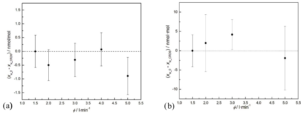
Figure 6. Differences between the reference (calculated) value of the water vapour mole fraction x_{w\_0} , and the water vapour mole fraction as measured by the CRDS analyser, x_{w\_CRDS} , at several flow rates, using 1.5 l·min -1 as the reference flow rate. Reported data refer to: (a) an absolute gas pressure of 800 hPa and a saturation temperature of -95.2\text{ }^{\circ}\text{C} that corresponds to an amount fraction x_{w\_0} of about 45.7 nmol·mol -1 ; (b) an absolute gas pressure of 1100 hPa and a saturation temperature of -74.9\text{ }^{\circ}\text{C} that corresponds to an amount fraction x_{w\_0} of about 1140 nmol·mol -1 . Error bars correspond to the square root of the sum of the variances of the instrument readings at the current and reference flow rate conditions.
