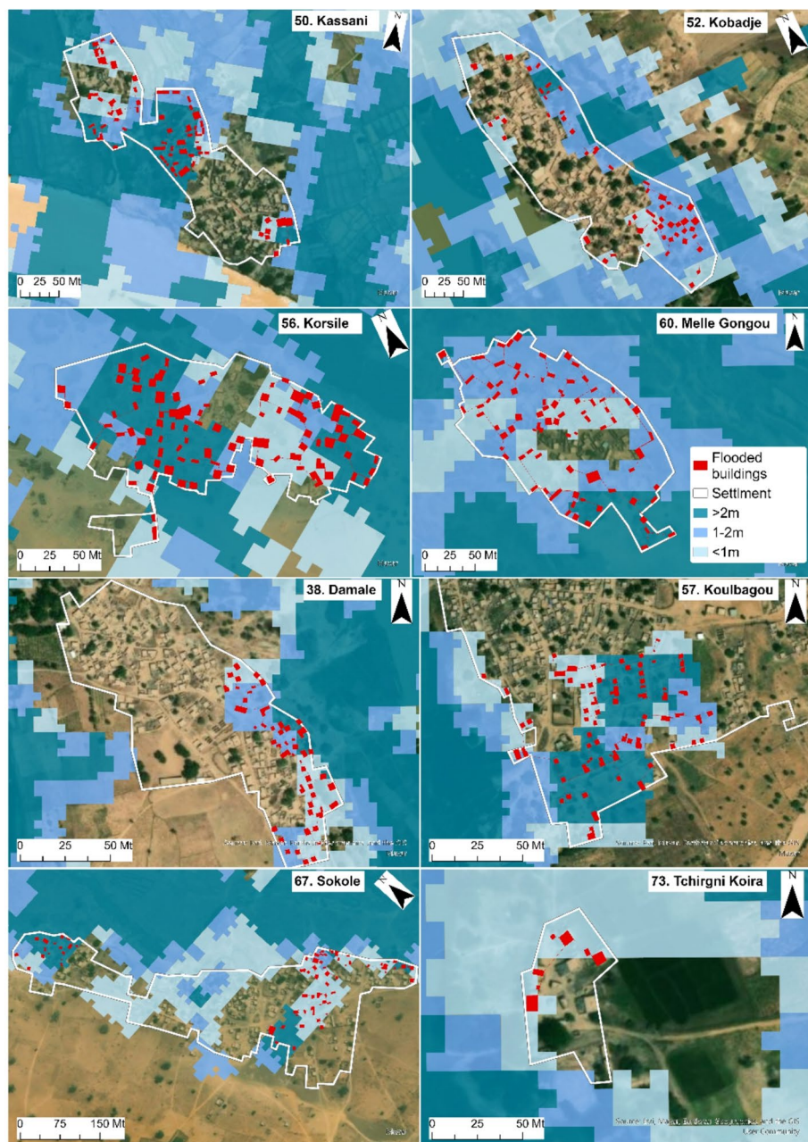
Fig. 13 Buildings likely affected by Guinean floods with a 10-year RP according to the water depth in Damale, Kassani, Kobadje, Korsile, Koulbagou, Melle Gongou, Sokole, and Tchirgni Koira
