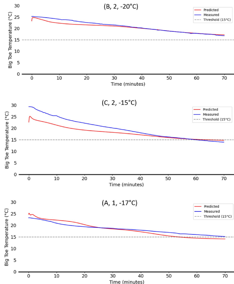
Fig. 4. Representative examples of accurate LSTM predictions. The network successfully captures both the shape of the temperature curve and the timing of the threshold-crossing event.
