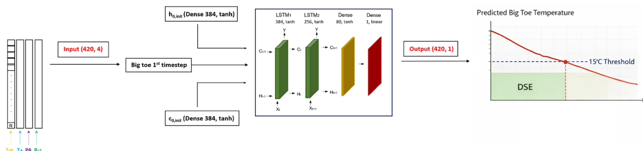
Fig. 1. Compact schematic of the final LSTM model for big toe temperature prediction, including hidden and cell state initialization from the first measured value.
