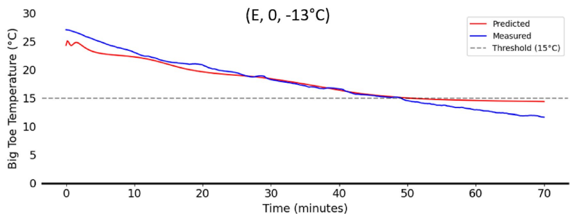
Fig. 5. Representative example of accurate LSTM predictions. The network successfully captures both the shape of the temperature curve and the timing of the threshold-crossing event.
