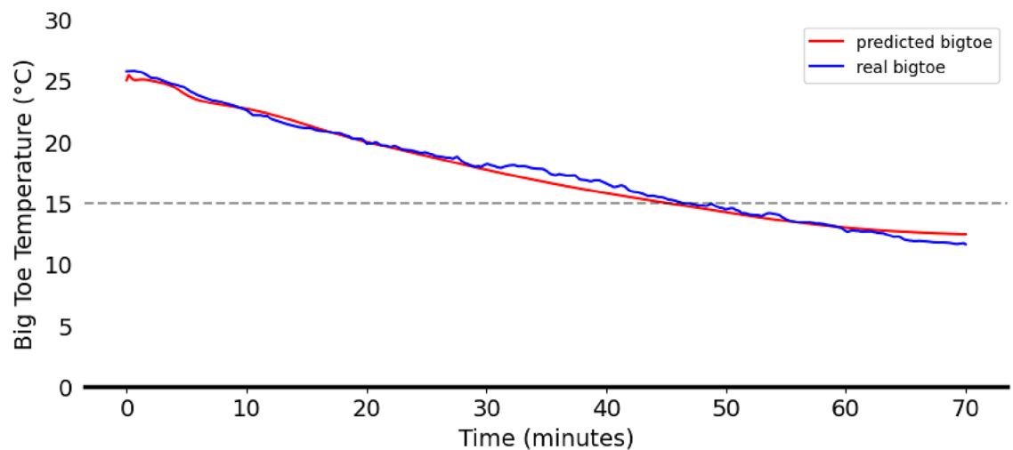
Fig. 7. Comparison between experimental and LSTM-predicted big toe temperature curves using synthetic mean skin temperature data generated by JOS-3.
