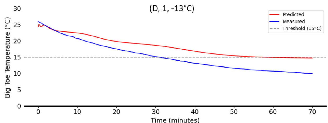
Fig. 6. Example of inaccurate prediction performance. The threshold crossing was not identified, although the overall temperature trajectory was correctly reproduced.
