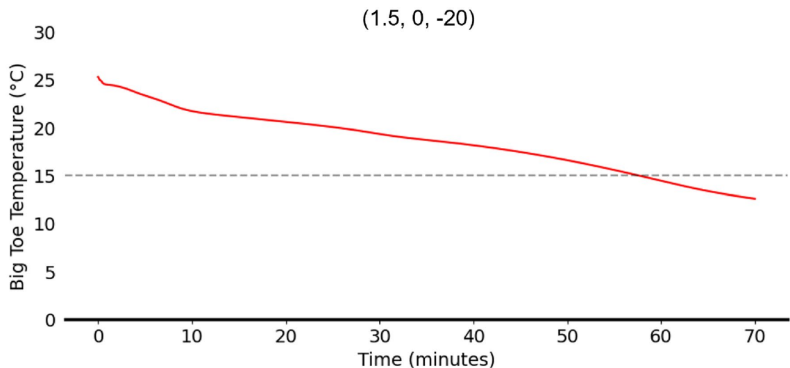
Fig. 8. LSTM prediction under stillness with high boot insulation and severe ambient temperature. The predicted time to reach the 15°C threshold is 57 minutes.
