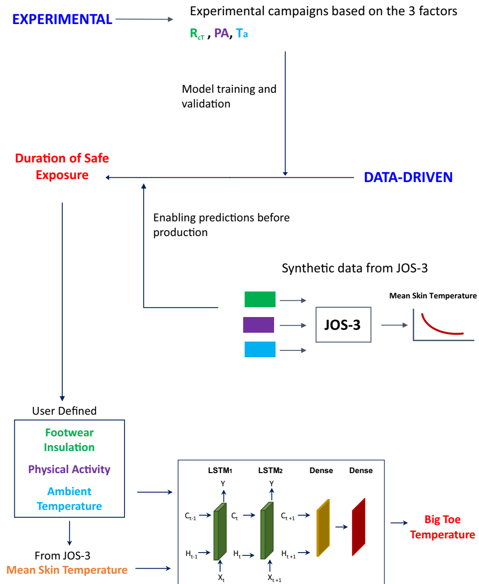
Fig. 2. Workflow of the project from experimental to synthetic data.
