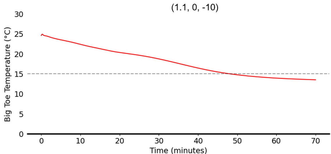
Fig. 11. LSTM prediction under stillness with low boot insulation at -10^{\circ}\text{C} . The predicted time to threshold is 47 minutes, highlighting the influence of insulation on toe cooling.
