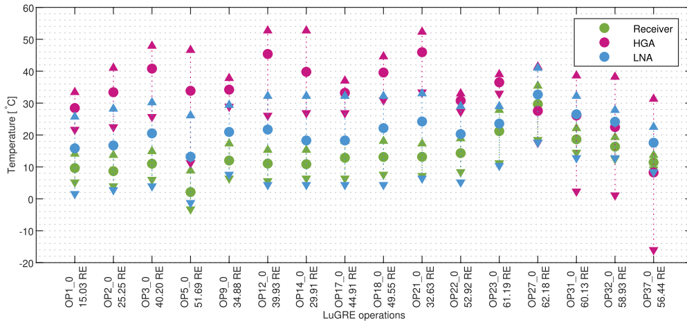
FIGURE 11 Temperatures observed during transit operations for the receiver, LNA, and HGA hardware
