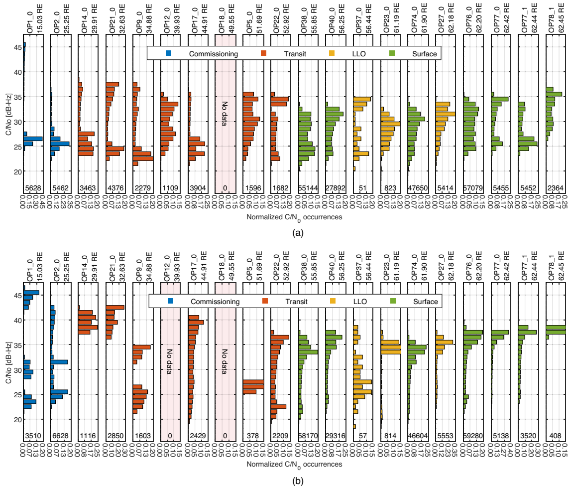
FIGURE 15 Normalized C/N_0 occurrences for GPS signals throughout mission operations. (a) GPS L1 C/A, (b) GPS L5Q.
