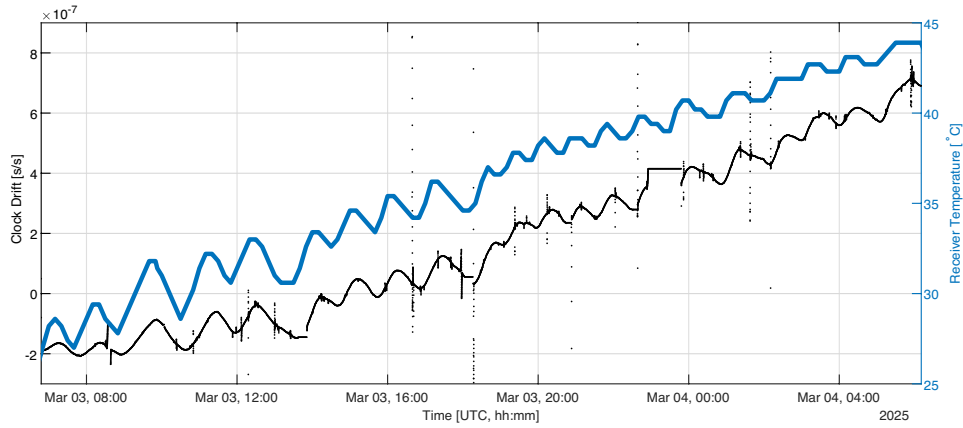
FIGURE 10 Receiver temperature and resulting clock drift behavior during early surface operations (as reported in the receiver POD telemetry)
