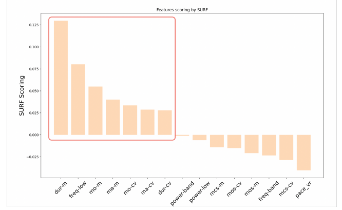
Fig. 2. Features rank scores yielded by the SURF algorithm. The selected features (positive scores) are squared in red.
