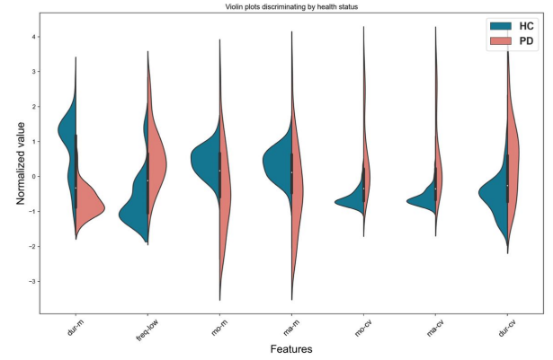
Fig. 3. Normalised violin plots of features in F_{opt} , estimated using the KDE approach, for PD and HC.
